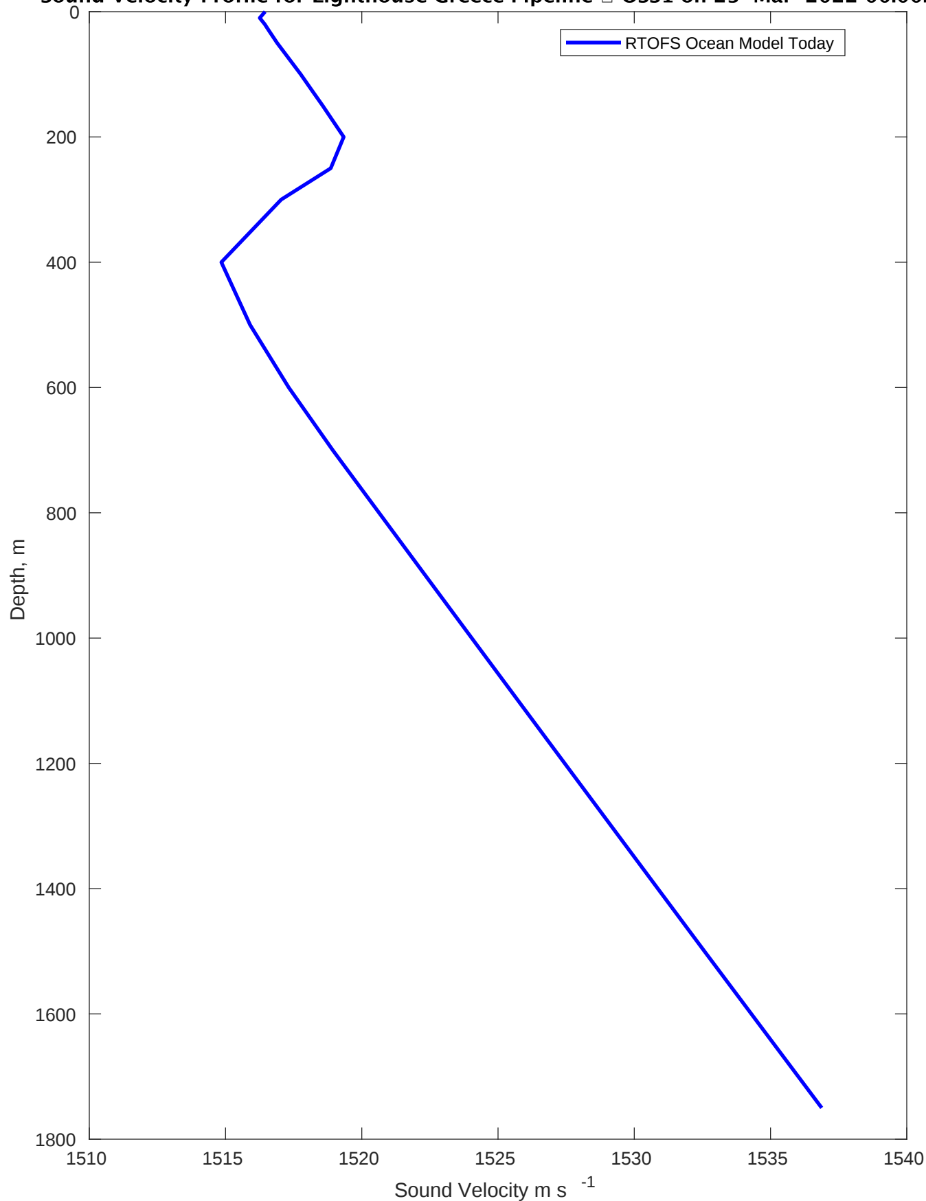
Sound Velocity Profile for Lighthouse Greece Pipeline □ OSS1 on 23-Mar-2022 00:00:00
