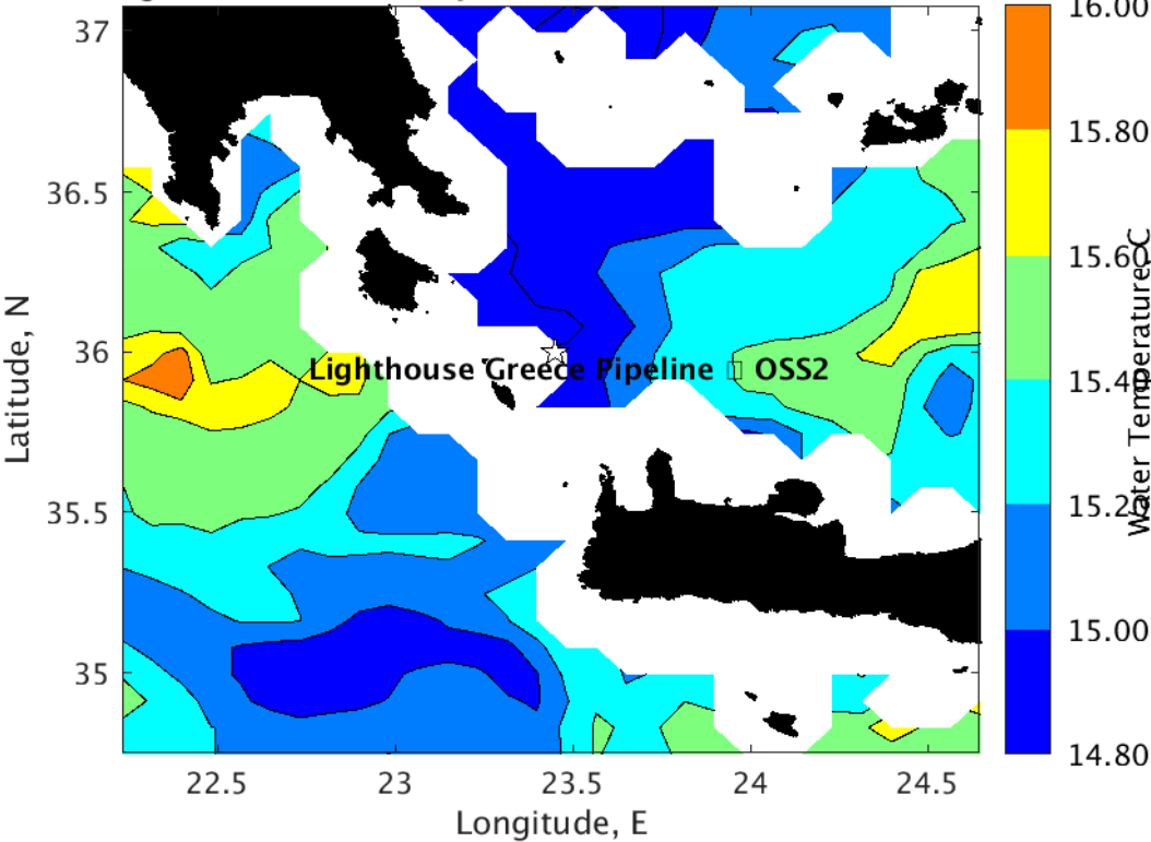
SST for Lighthouse Greece Pipeline □ OSS2 at 23-Mar-2022 00:00:00
