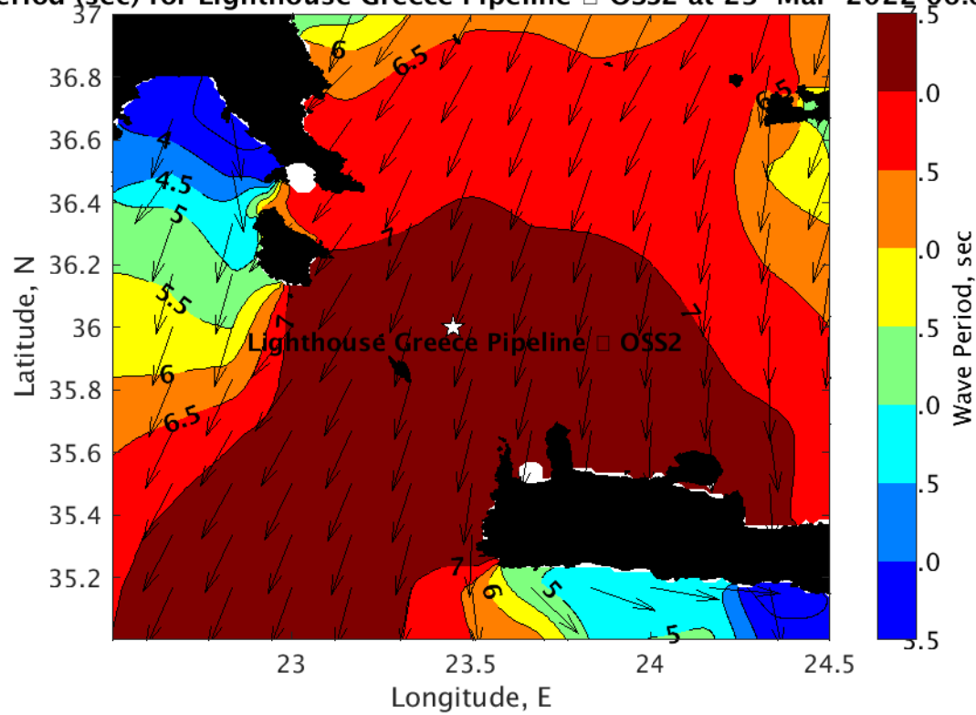
Wave Period (sec) for Lighthouse Greece Pipeline □ OSS2 at 23-Mar-2022 06:00:00
