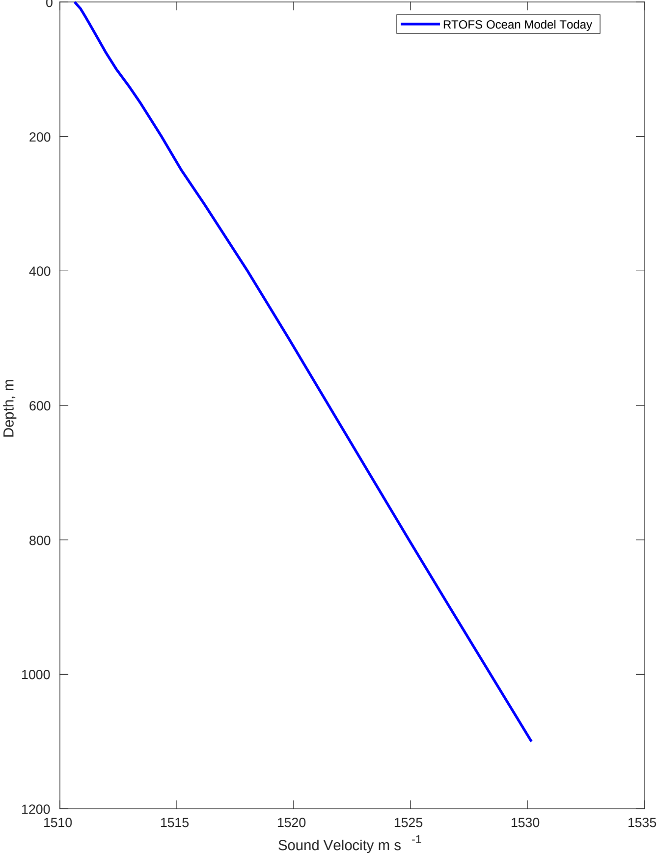
Sound Velocity Profile for Lighthouse Greece Pipeline □ OSS2 on 23-Mar-2022 00:00:00
