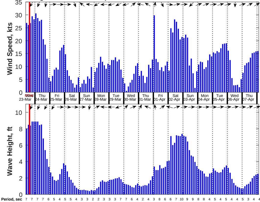
Wind & Wave Forecast for Lighthouse Greece Pipeline □ OSS2 from 23-Mar-2022 09:00:00 to 08-Apr-2022 06:00:00
