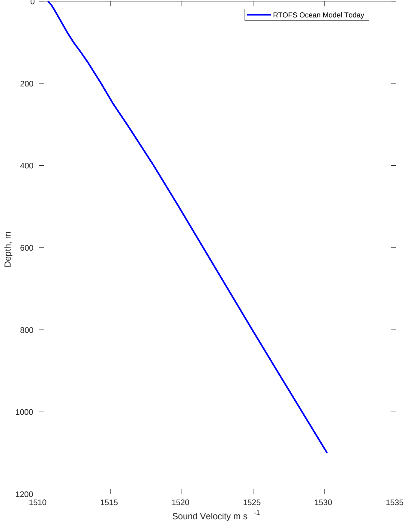
Sound Velocity Profile for Lighthouse Greece Pipeline □ OSS3 on 23-Mar-2022 00:00:00
