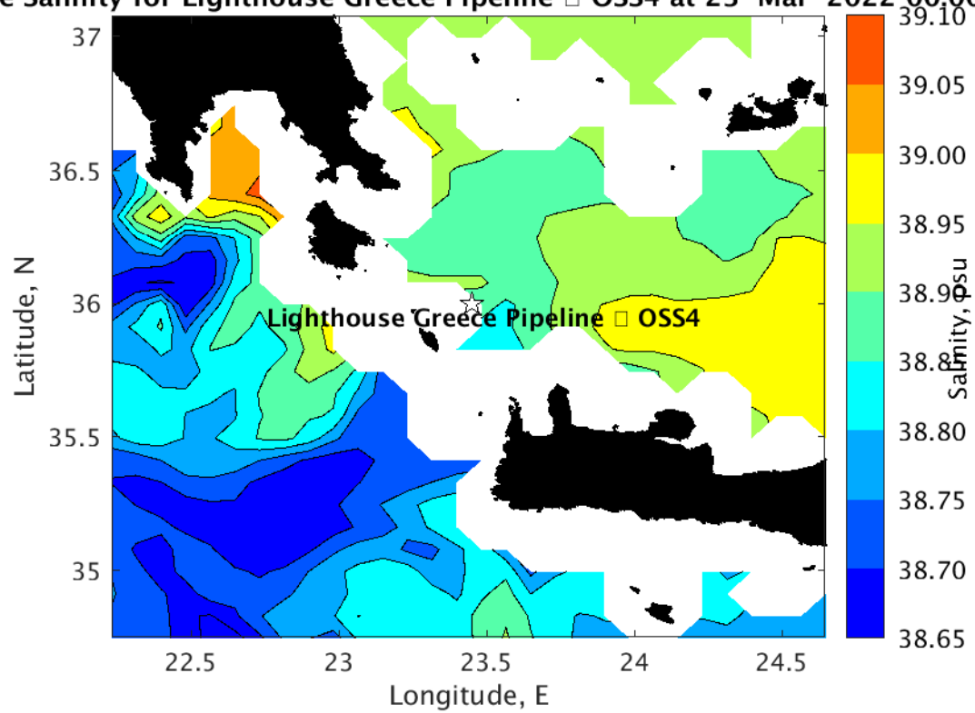
Sea Salinity for Lighthouse Greece Pipeline □ OSS4 at 23-Mar-2022 00:00:00
