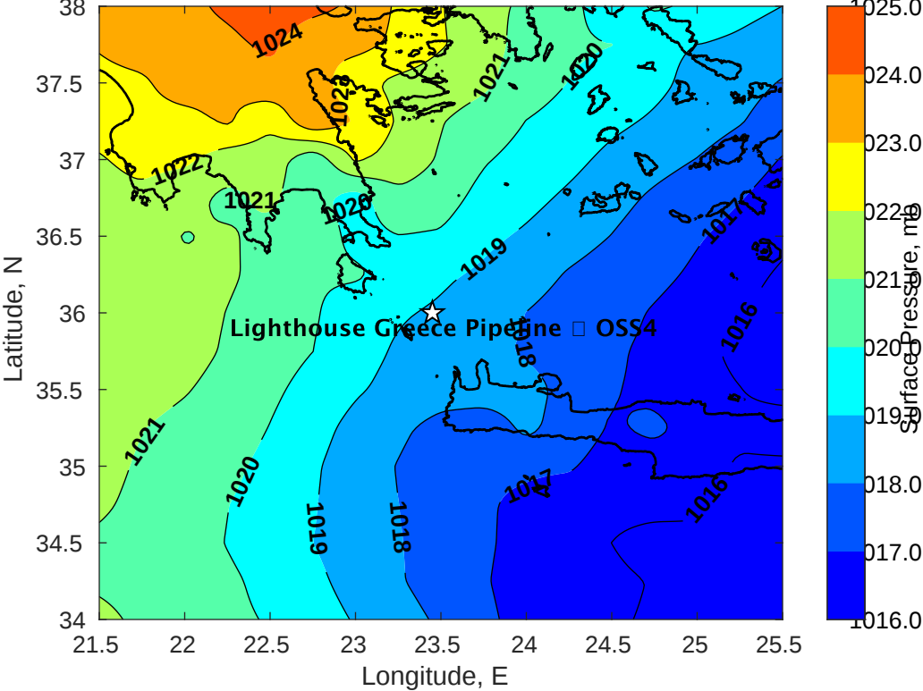
Surface Pressure (mb) for Lighthouse Greece Pipeline □ OSS4 at 23-Mar-2022 06:00:00
