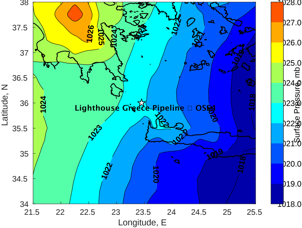
Surface Pressure (mb) for Lighthouse Greece Pipeline □ OSS4 at 24-Mar-2022 03:00:00
