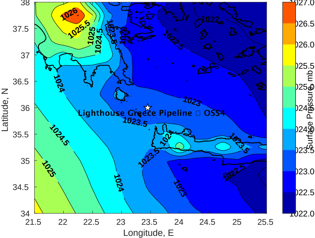
Surface Pressure (mb) for Lighthouse Greece Pipeline □ OSS4 at 25-Mar-2022 03:00:00
