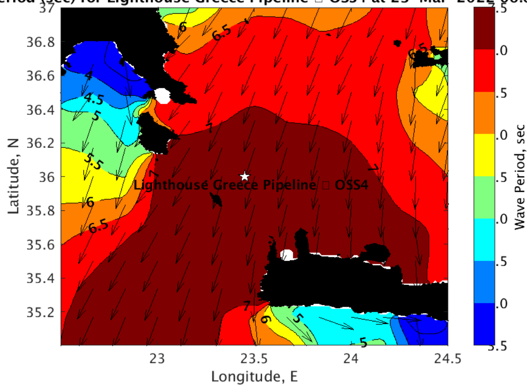
Wave Period (sec) for Lighthouse Greece Pipeline □ OSS4 at 23-Mar-2022 06:00:00
