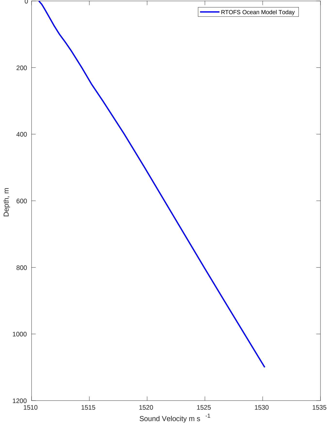
Sound Velocity Profile for Lighthouse Greece Pipeline □ OSS4 on 23-Mar-2022 00:00:00
