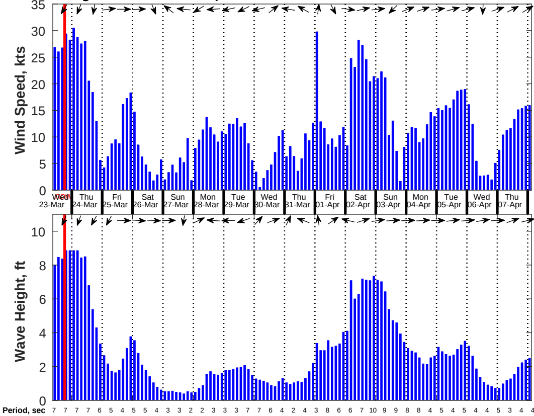
Wind & Wave Forecast for Lighthouse Greece Pipeline □ OSS4 from 23-Mar-2022 09:00:00 to 08-Apr-2022 06:00:00
