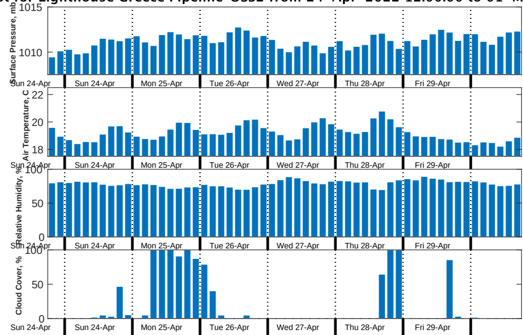
Met Forecast for Lighthouse Greece Pipeline-OSS2 from 24-Apr-2022 12:00:00 to 01-May-2022 12:00:00
