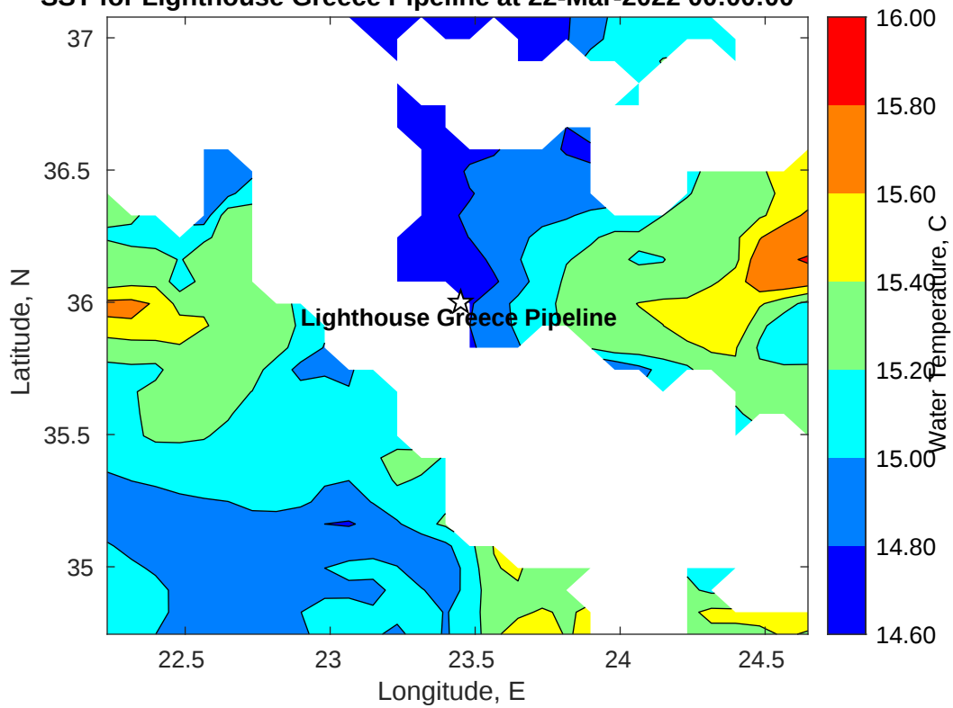
SST for Lighthouse Greece Pipeline at 22-Mar-2022 00:00:00
