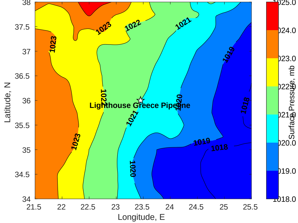
Surface Pressure (mb) for Lighthouse Greece Pipeline at 22-Mar-2022 12:00:00
