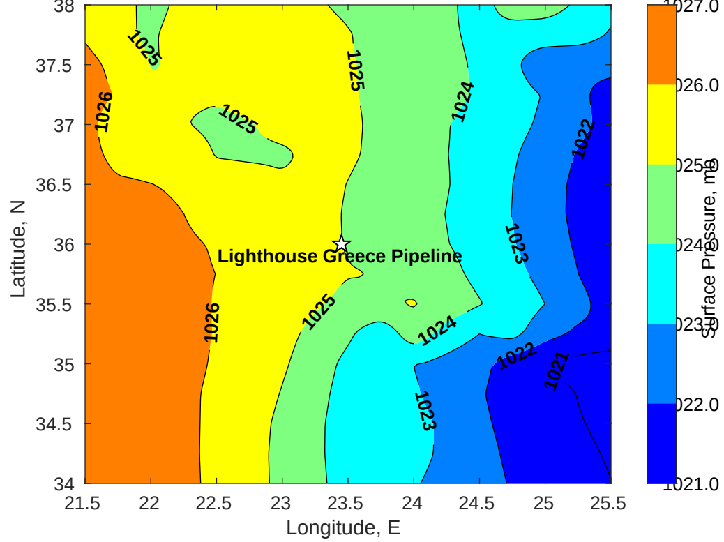
Surface Pressure (mb) for Lighthouse Greece Pipeline at 24-Mar-2022 09:00:00
