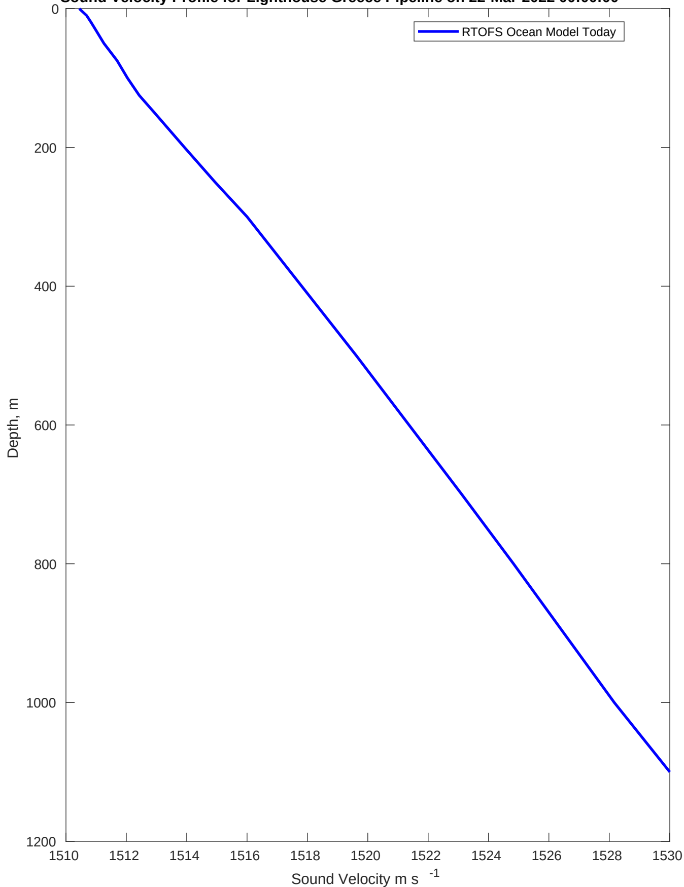
Sound Velocity Profile for Lighthouse Greece Pipeline on 22-Mar-2022 00:00:00
