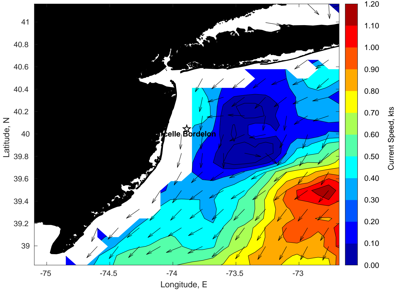
Surface Currents for Marcelle Bordelon at 06-Feb-2024 00:00:00
