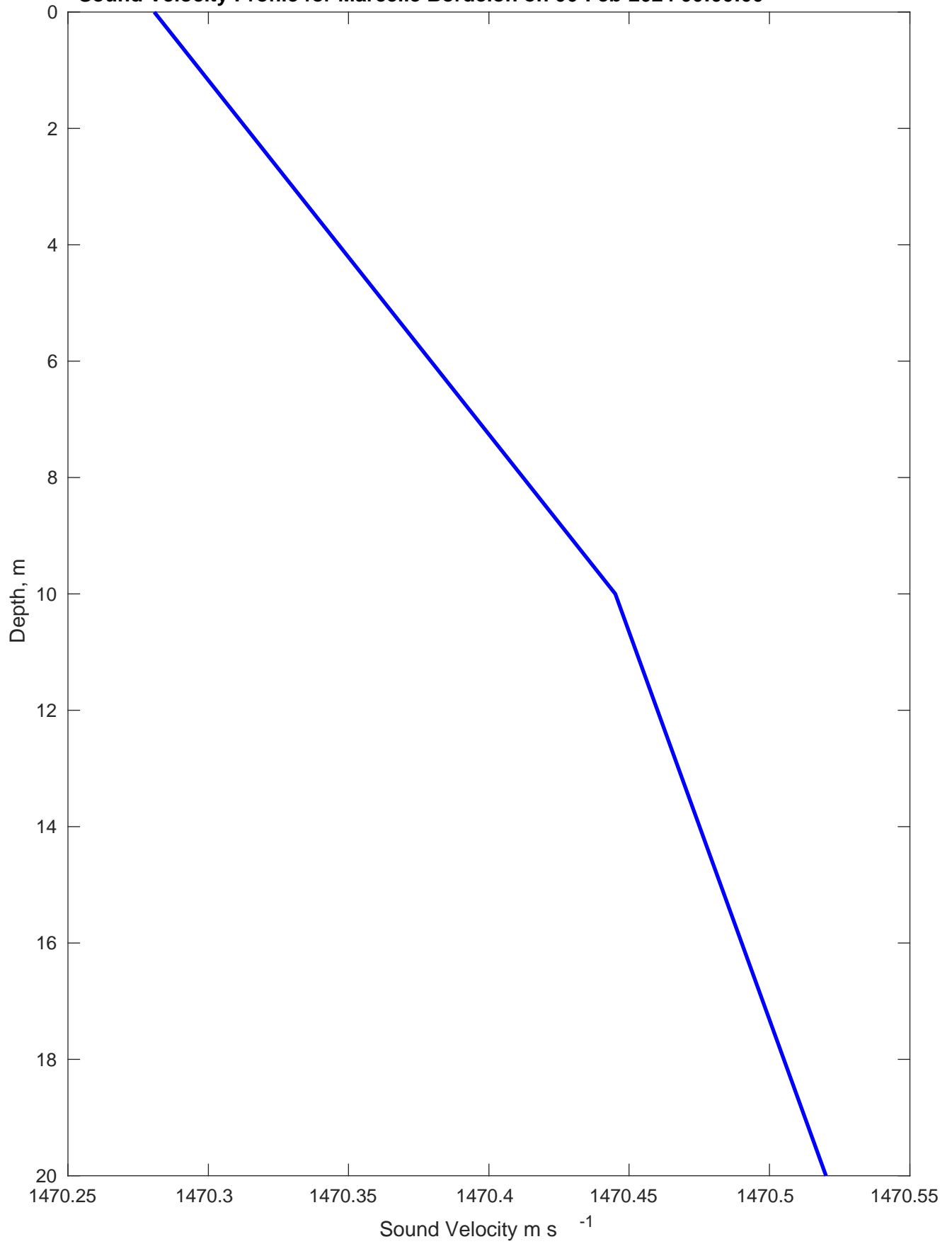
Sound Velocity Profile for Marcelle Bordelon on 06-Feb-2024 00:00:00
