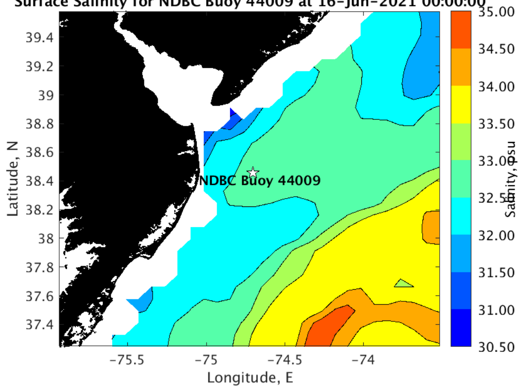
Surface Salinity for NDBC Buoy 44009 at 16-Jun-2021 00:00:00
