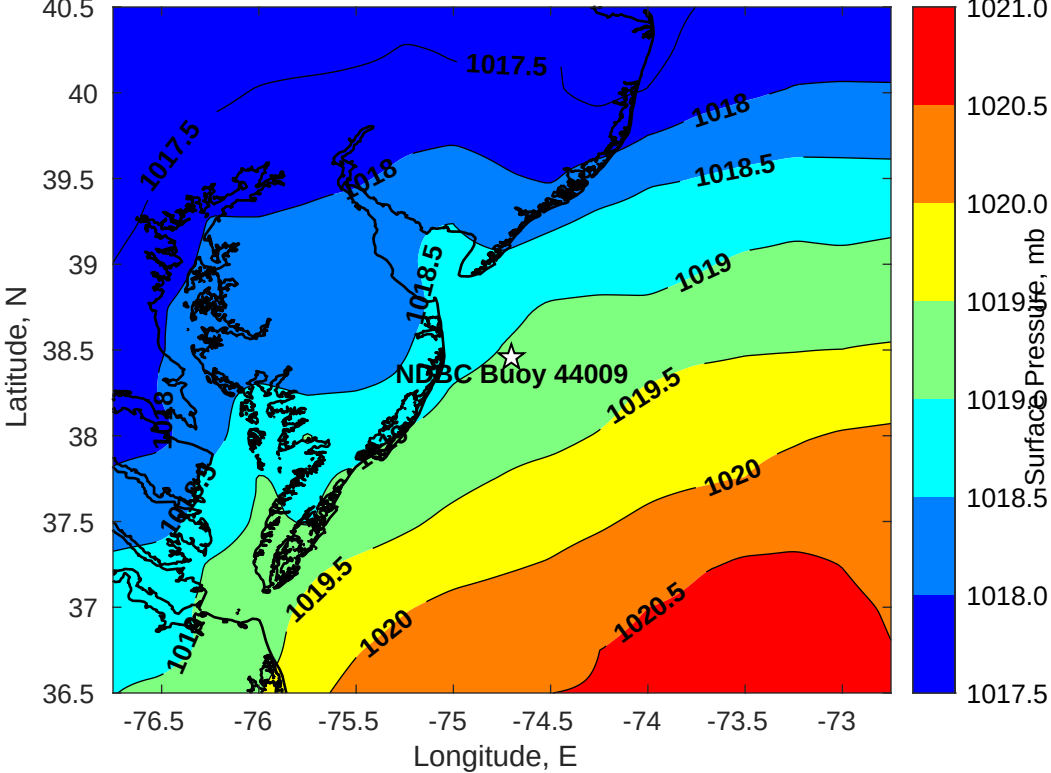
Surface Pressure (mb) for NDBC Buoy 44009 at 18-Jun-2021 15:00:00
