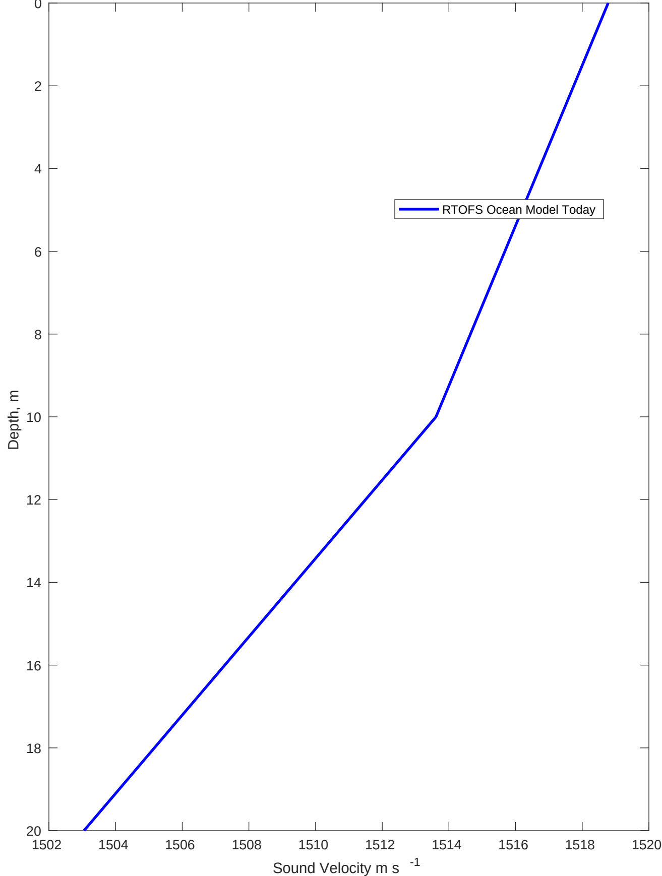
Sound Velocity Profile for NDBC Buoy 44009 on 16-Jun-2021 00:00:00
