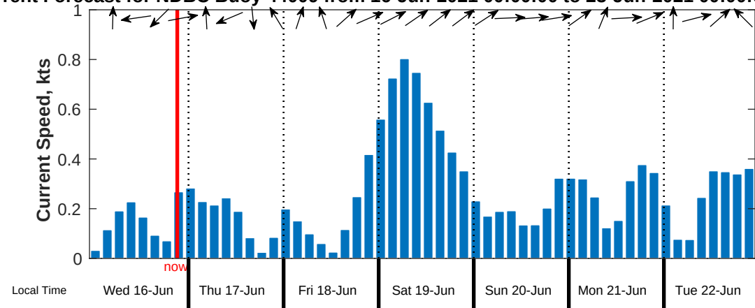
Current Forecast for NDBC Buoy 44009 from 16-Jun-2021 00:00:00 to 23-Jun-2021 00:00:00
