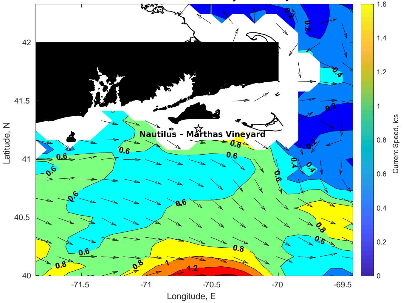
Surface Currents for Nautilus - Marthas Vineyard at 25-Jun-2024 00:00:00
