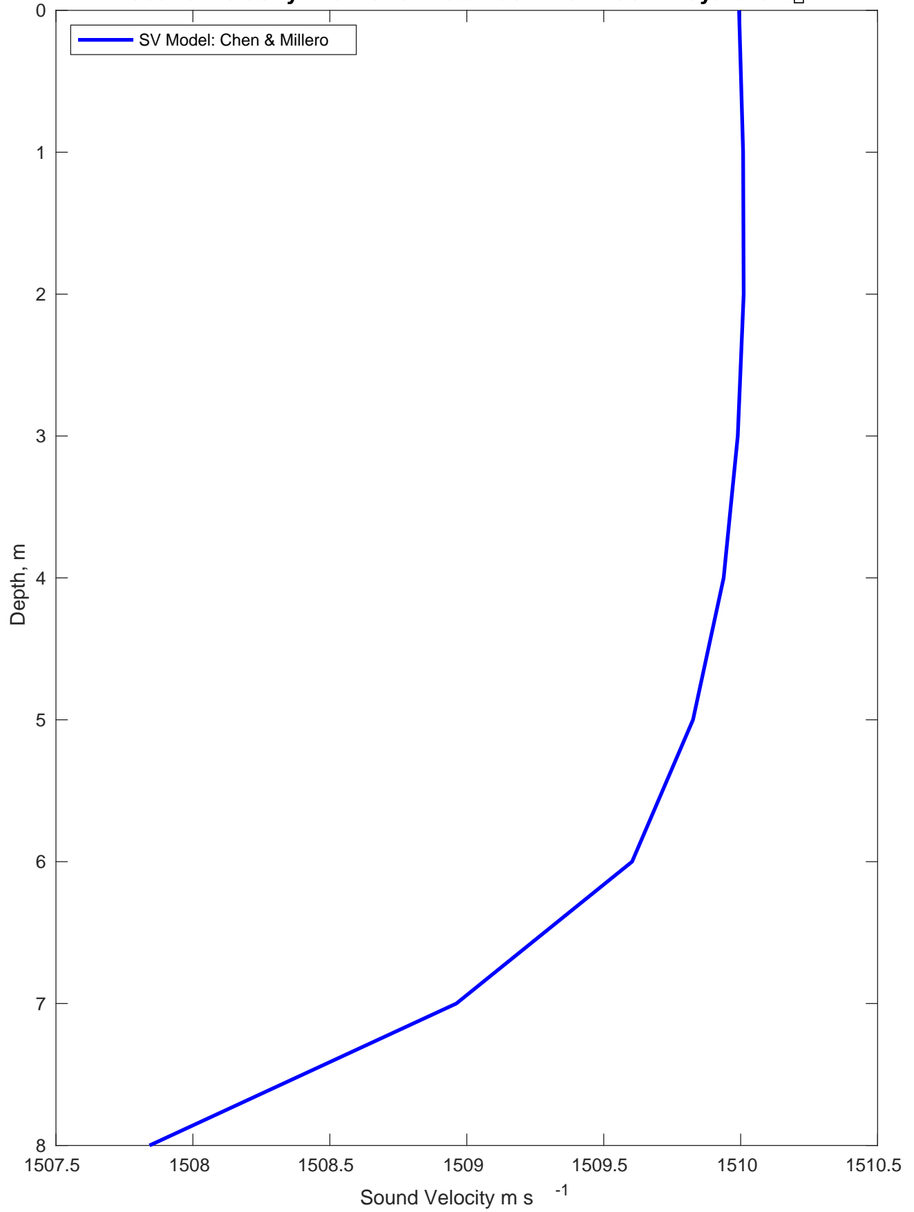
Sound Velocity Profile for Nautilus - Marthas Vineyard on [ ]
