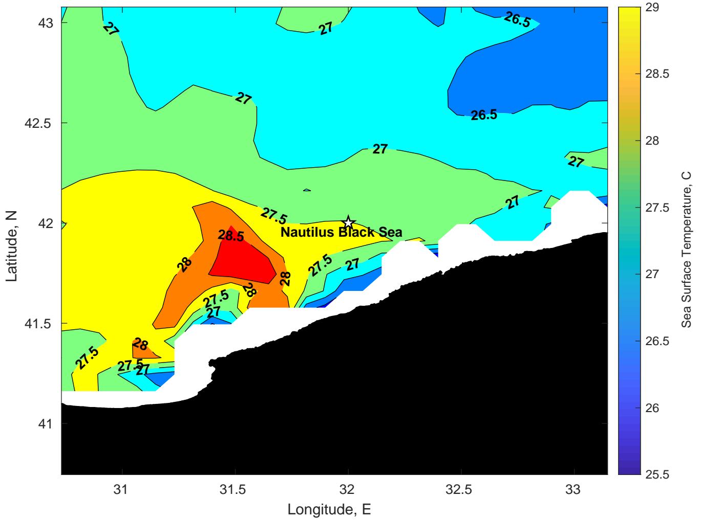
SST for Nautilus Black Sea at 28-Jul-2024 00:00:00
