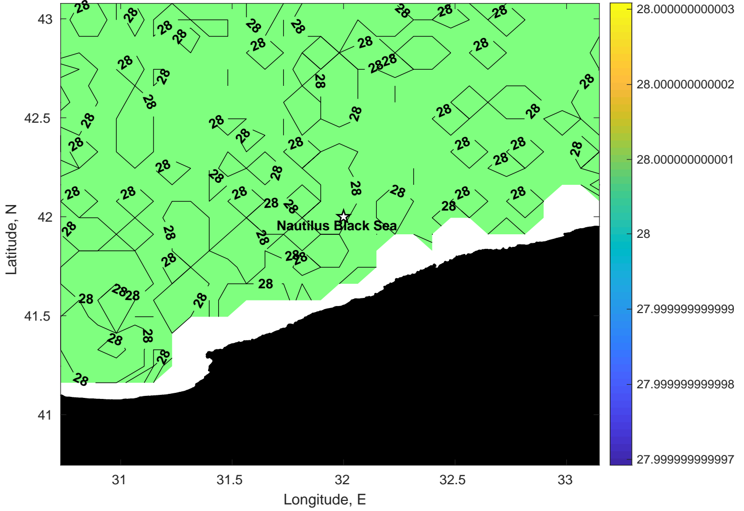
Surface Salinity for Nautilus Black Sea at 28-Jul-2024 00:00:00
