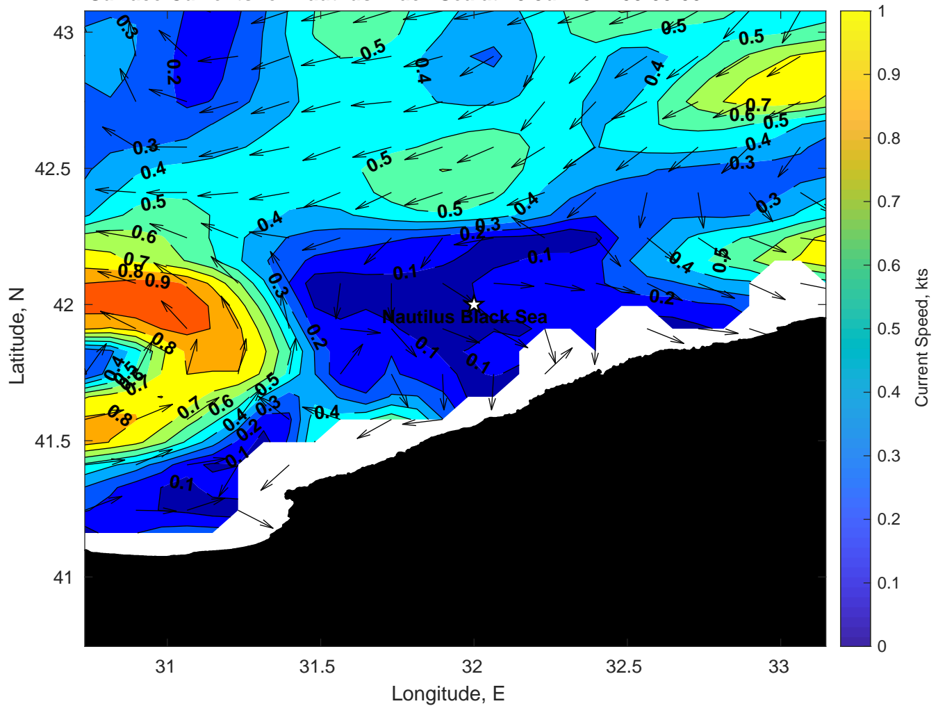
Surface Currents for Nautilus Black Sea at 28-Jul-2024 00:00:00
