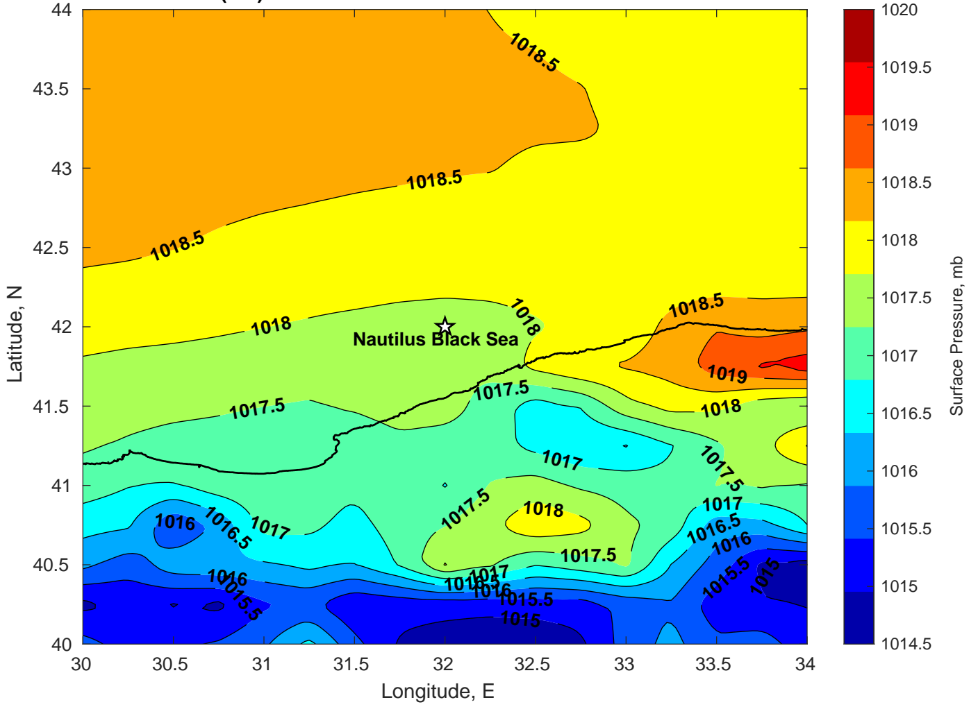
Surface Pressure (mb) for Nautilus Black Sea at 28-Jul-2024 12:00:00
