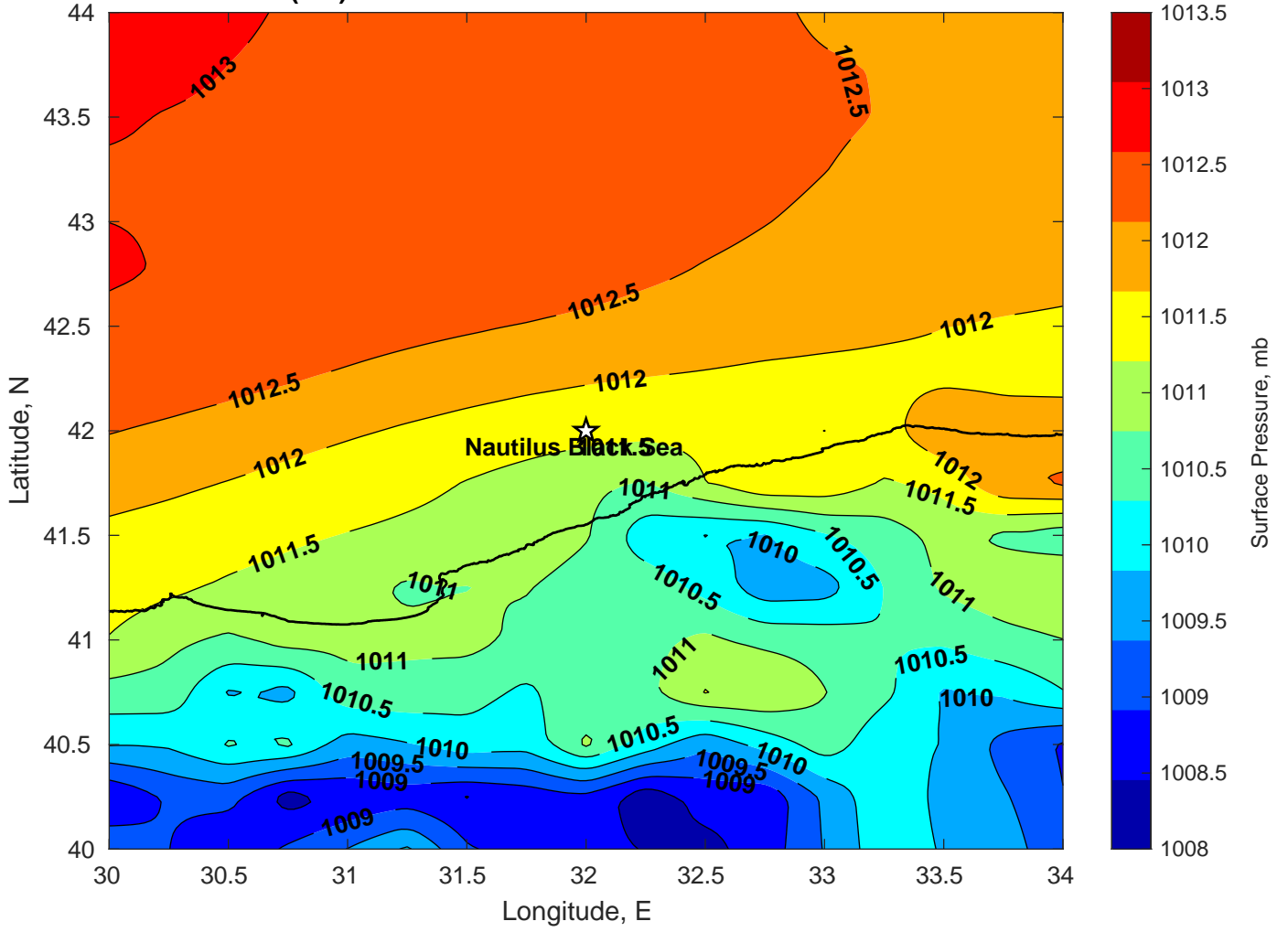
Surface Pressure (mb) for Nautilus Black Sea at 29-Jul-2024 12:00:00
