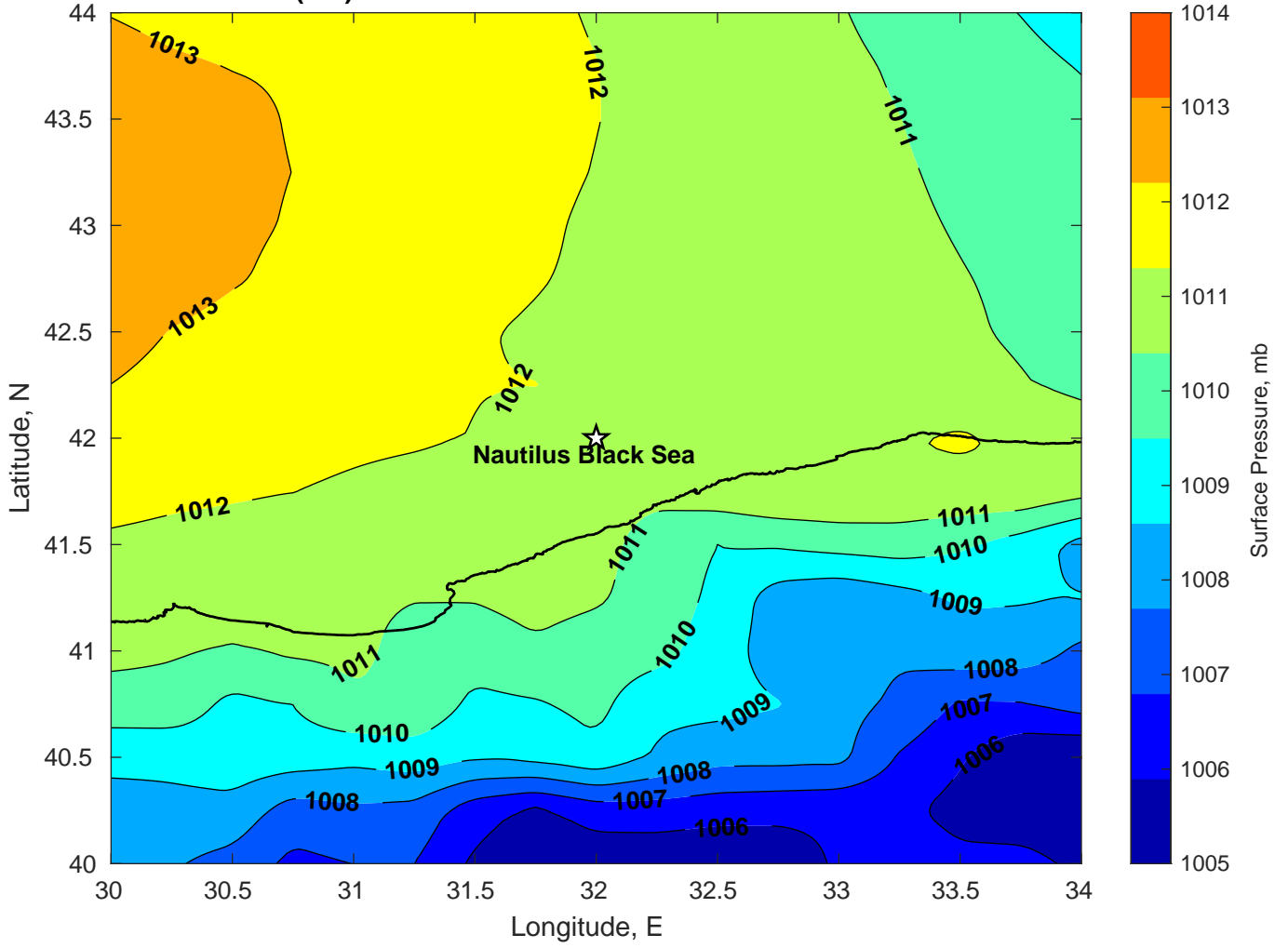
Surface Pressure (mb) for Nautilus Black Sea at 30-Jul-2024 12:00:00
