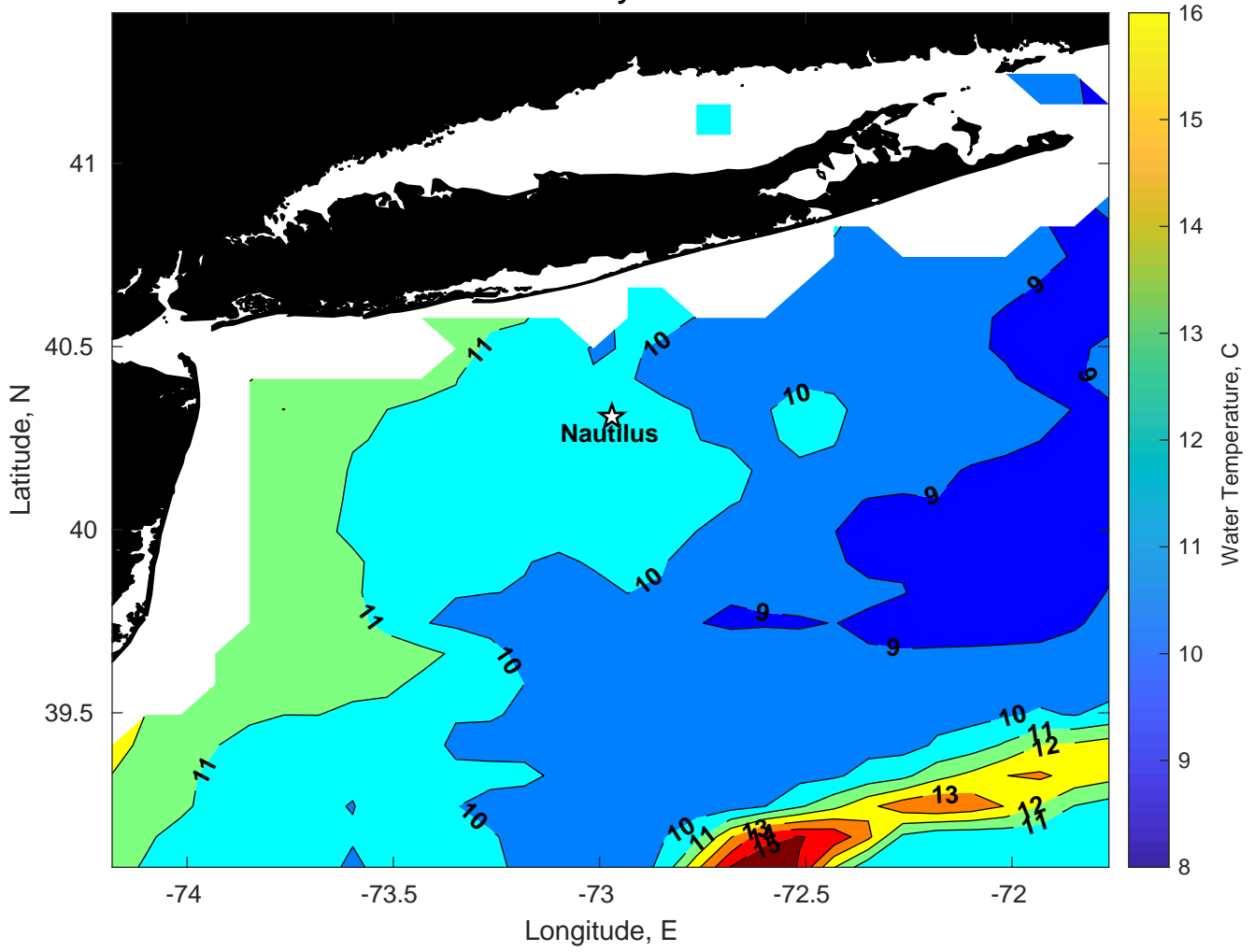
SST for Nautilus at 04-May-2024 00:00:00
