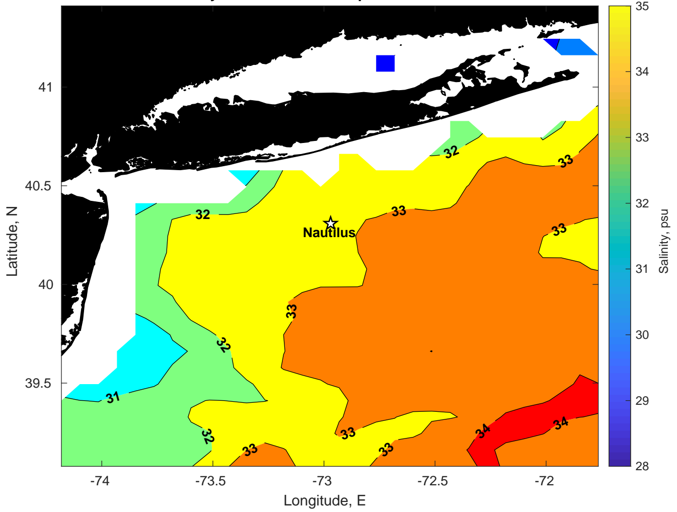
Surface Salinity for Nautilus at 28-Apr-2024 00:00:00
