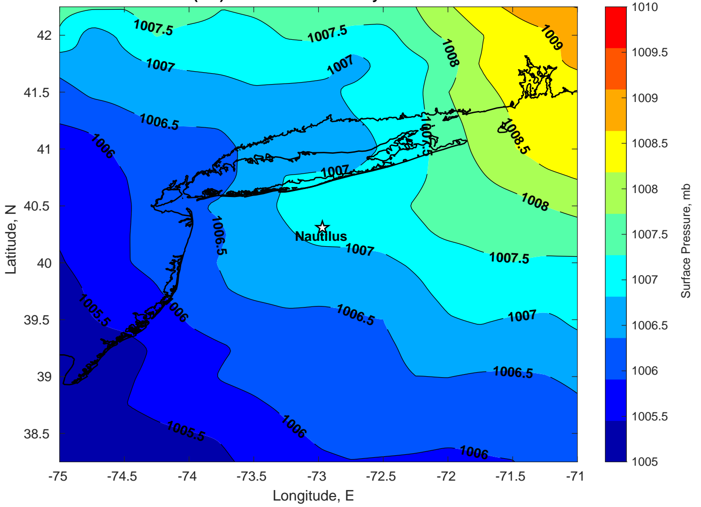
Surface Pressure (mb) for Nautilus at 10-May-2024 00:00:00
