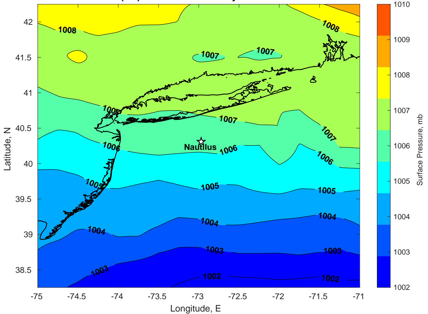
Surface Pressure (mb) for Nautilus at 10-May-2024 18:00:00
