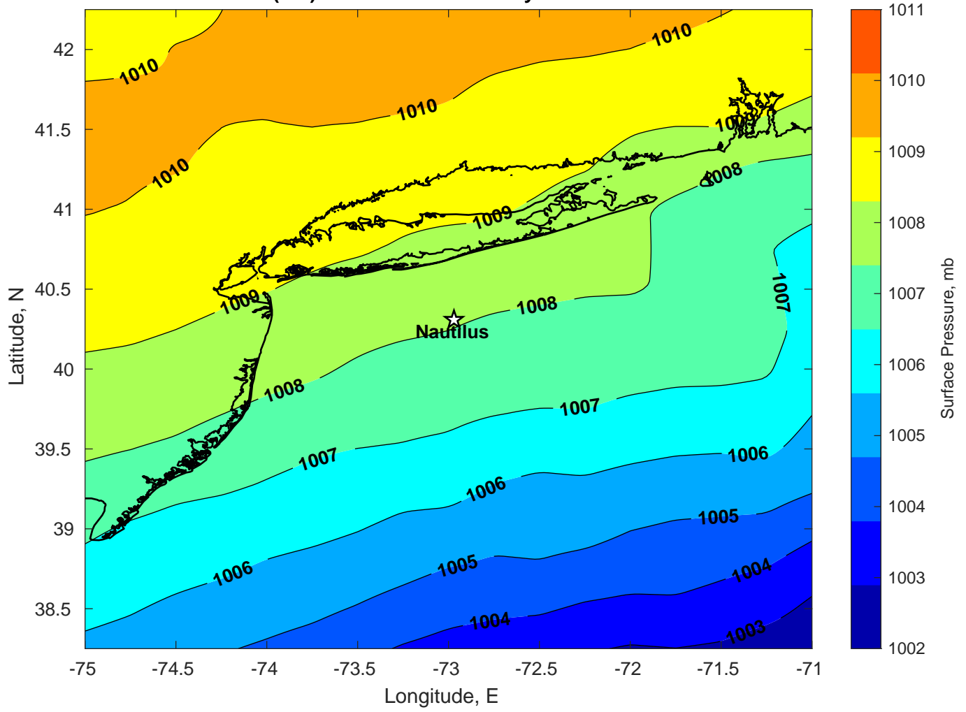
Surface Pressure (mb) for Nautilus at 11-May-2024 06:00:00
