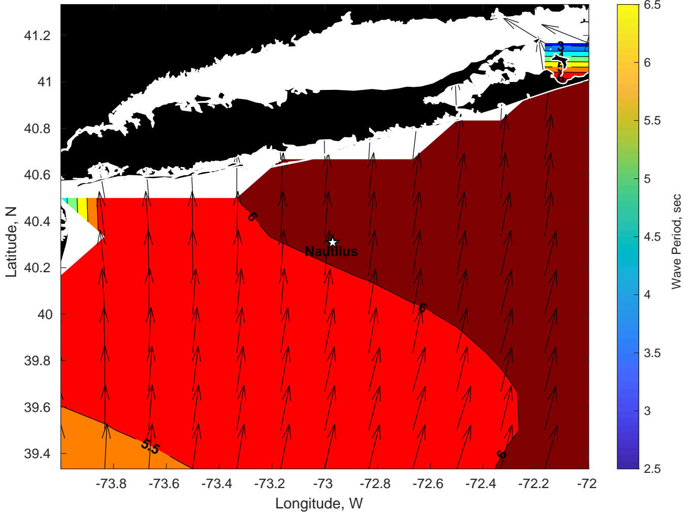
Wave Period (sec) for Nautilus at 02-May-2024 00:00:00
