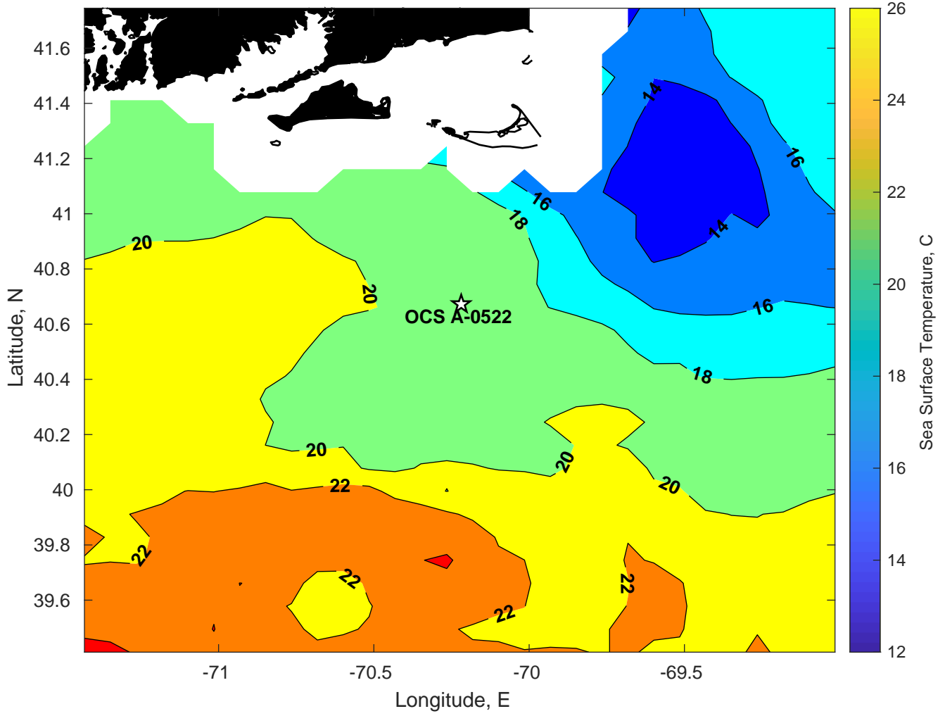
SST for OCS A-0522 at 24-Jun-2024 00:00:00
