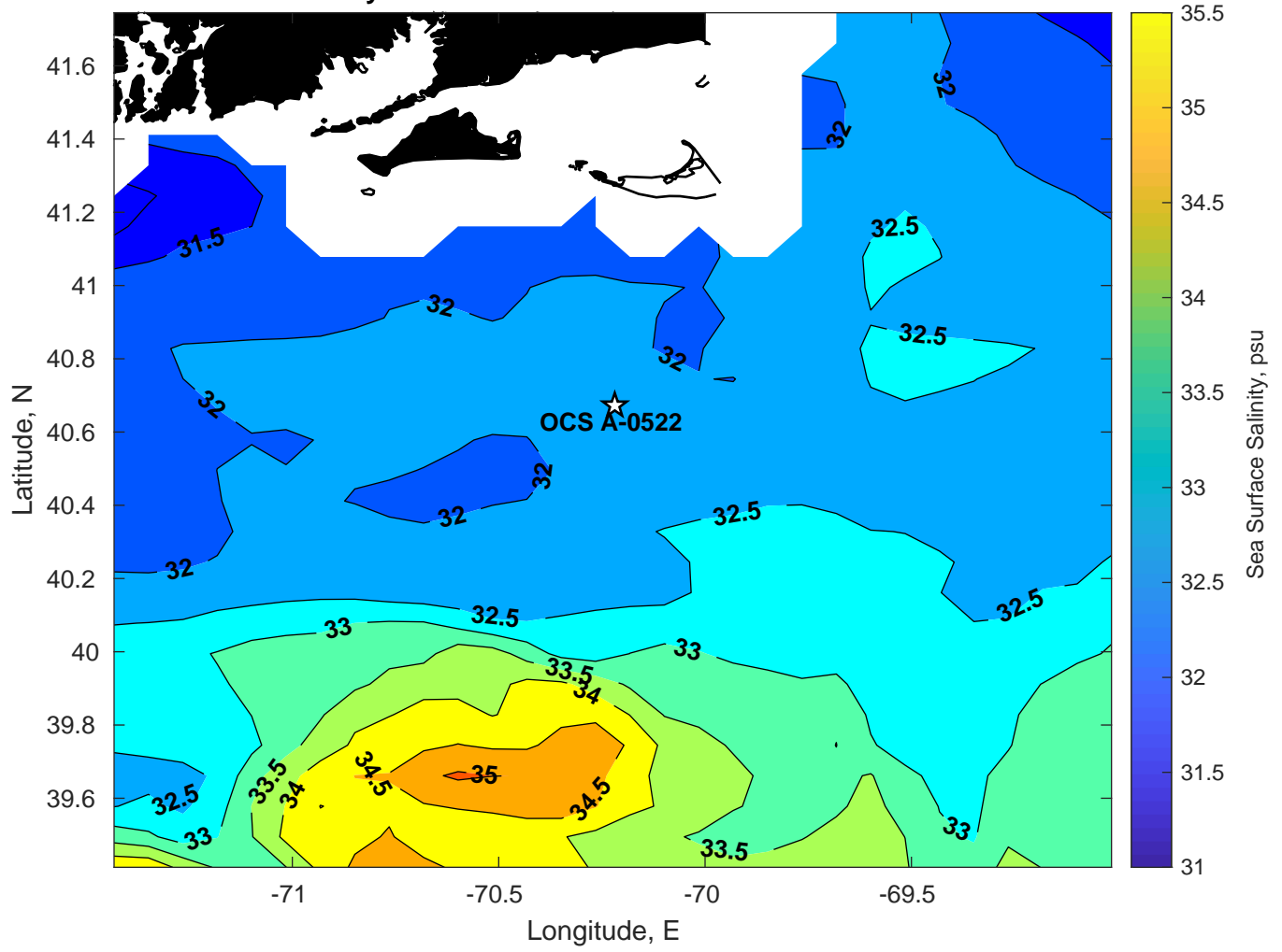
Surface Salinity for OCS A-0522 at 24-Jun-2024 00:00:00
