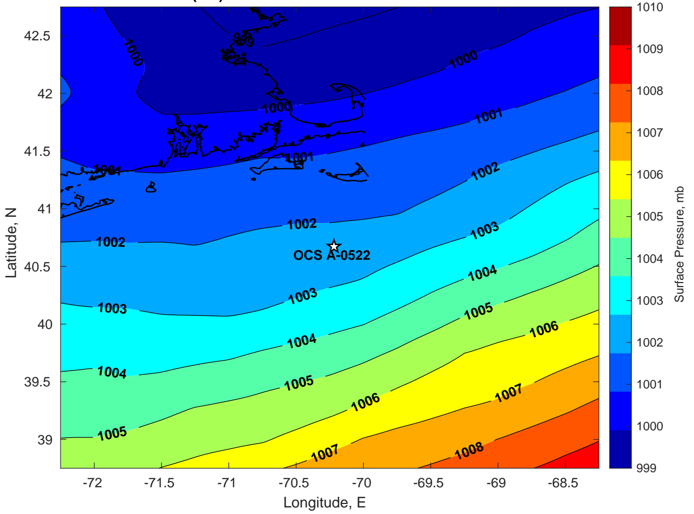
Surface Pressure (mb) for OCS A-0522 at 24-Jun-2024 12:00:00
