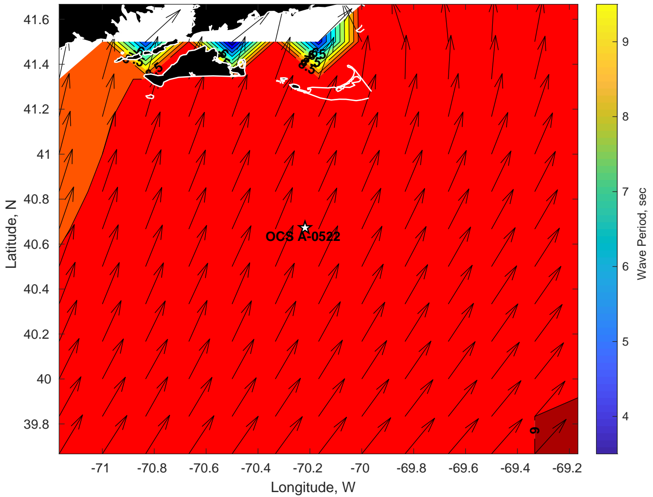
Wave Period (sec) for OCS A-0522 at 24-Jun-2024 18:00:00
