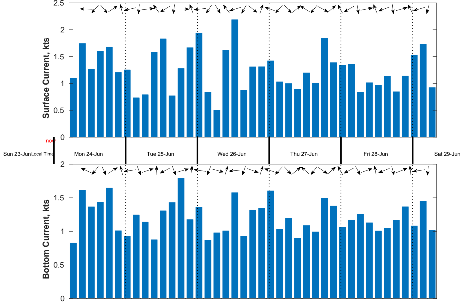
Surface Current Forecast for OCS A-0522 from 24-Jun-2024 21:00:00 to 30-Jun-2024 00:00:00
