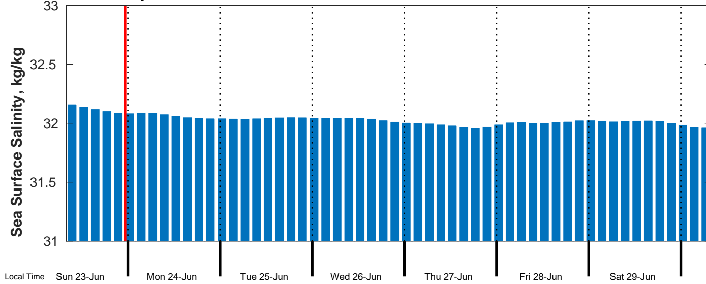
Sea Surface Salinity Forecast for OCS A-0522 from 24-Jun-2024 00:00:00 to 01-Jul-2024 00:00:00
