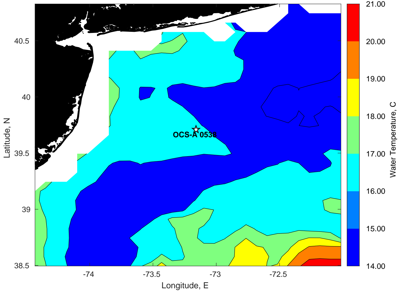
SST for OCS-A 0538 at 10-Jun-2023 00:00:00
