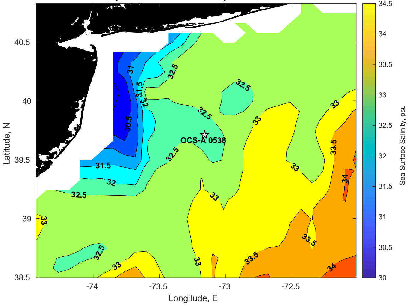
Surface Salinity for OCS-A 0538 at 13-Sep-2024 00:00:00
