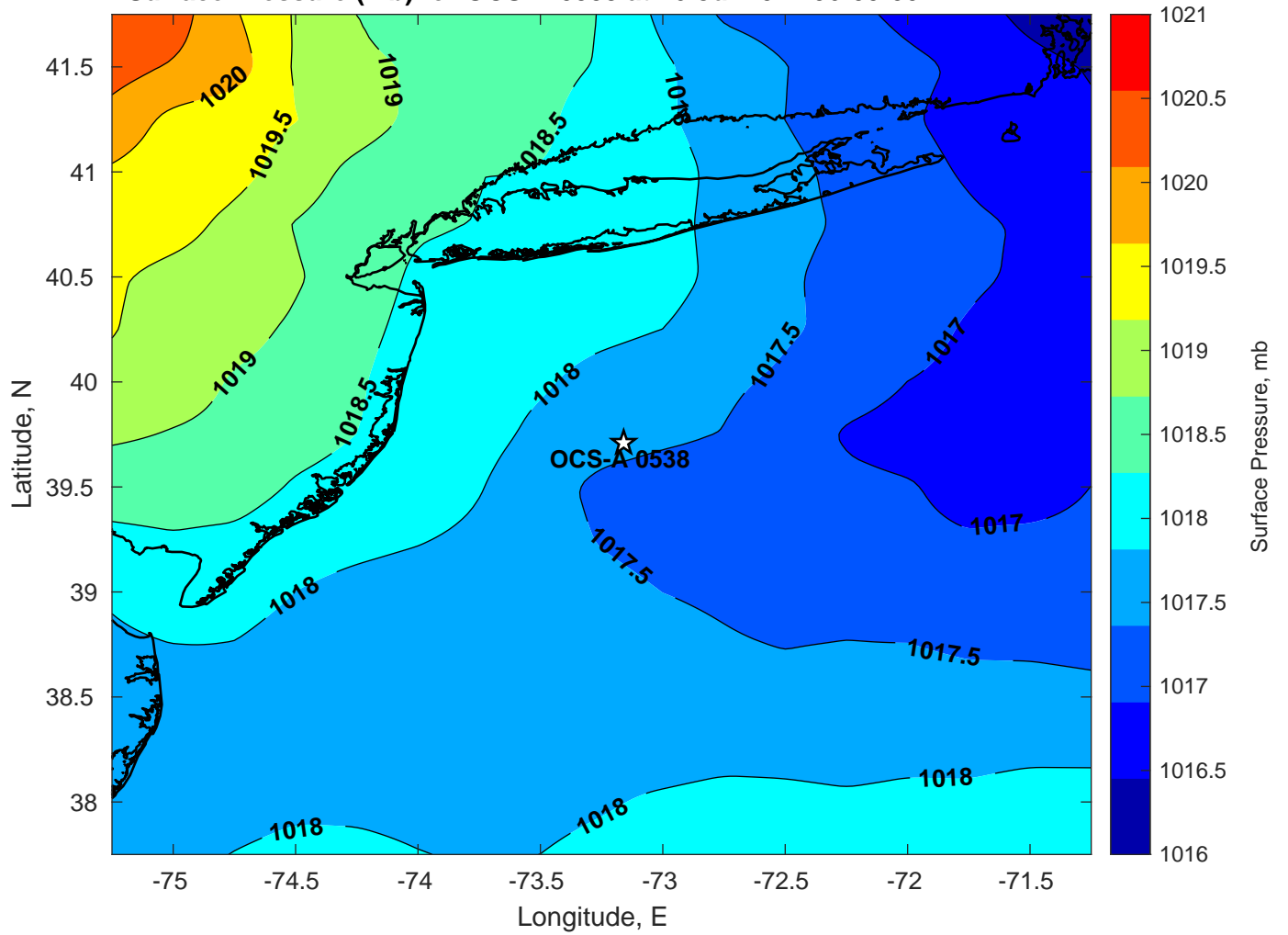
Surface Pressure (mb) for OCS-A 0538 at 26-Jul-2024 06:00:00
