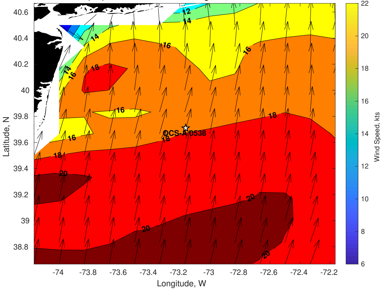
Winds (kts) for OCS-A 0538 at 03-Aug-2024 00:00:00
