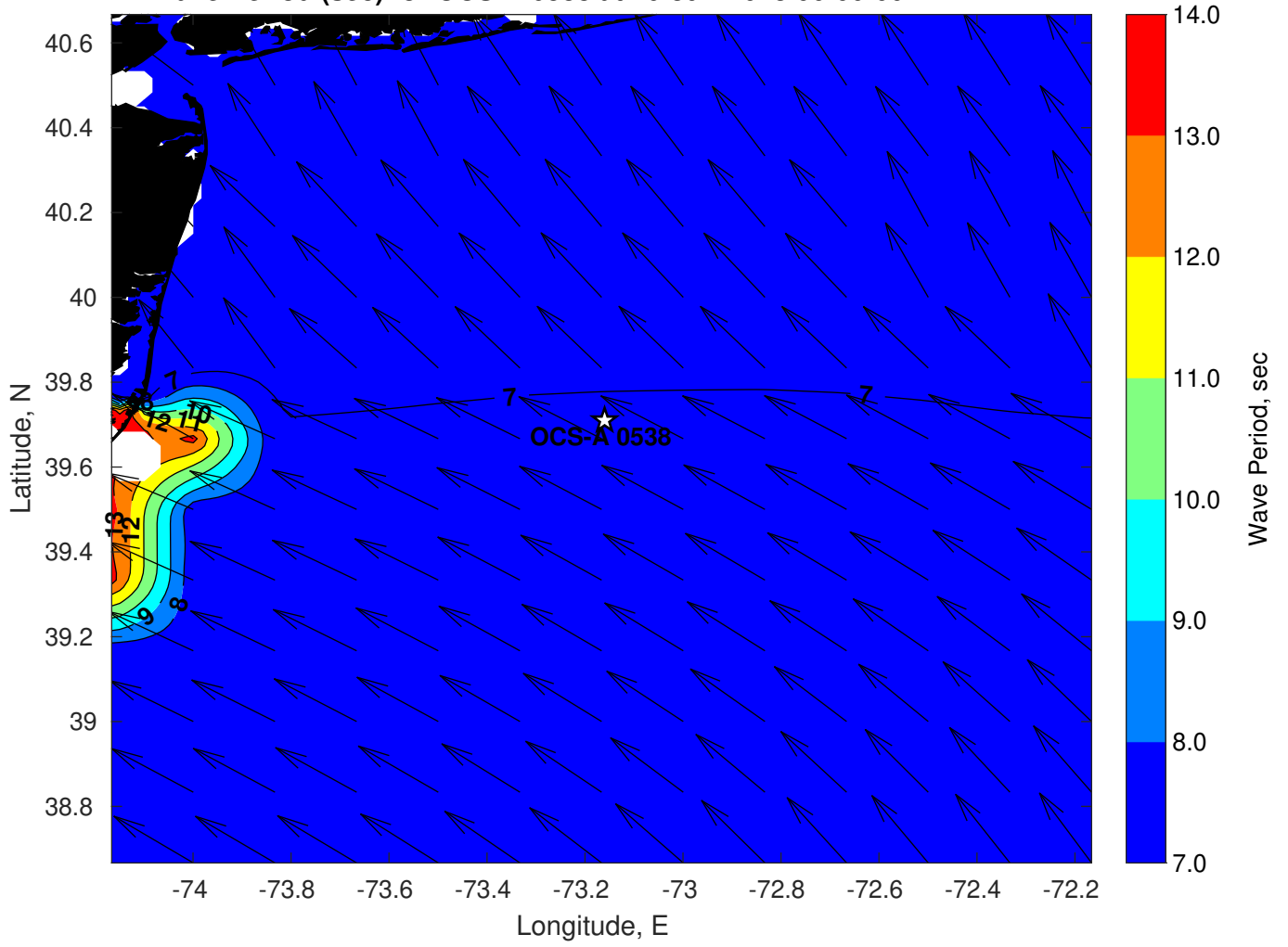
Wave Period (sec) for OCS-A 0538 at 10-Jun-2023 06:00:00
