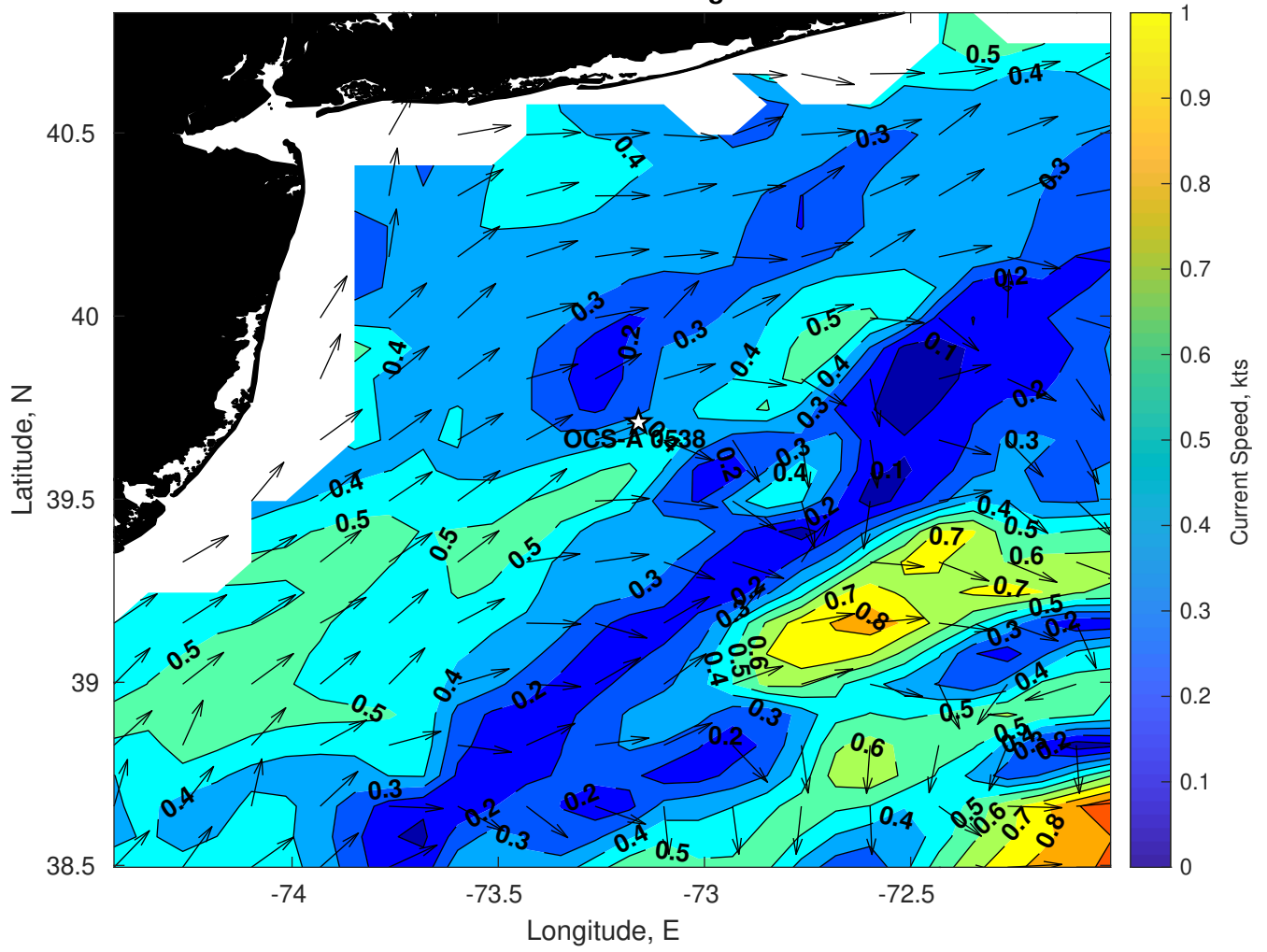
Surface Currents for OCS-A 0538 at 02-Aug-2024 00:00:00
