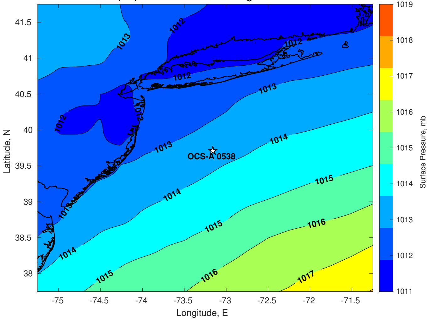
Surface Pressure (mb) for OCS-A 0538 at 04-Aug-2024 18:00:00
