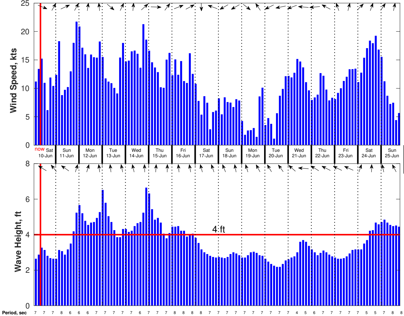
Wind & Wave Forecast for OCS-A 0538 from 10-Jun-2023 02:00:00 to 26-Jun-2023 02:00:00
