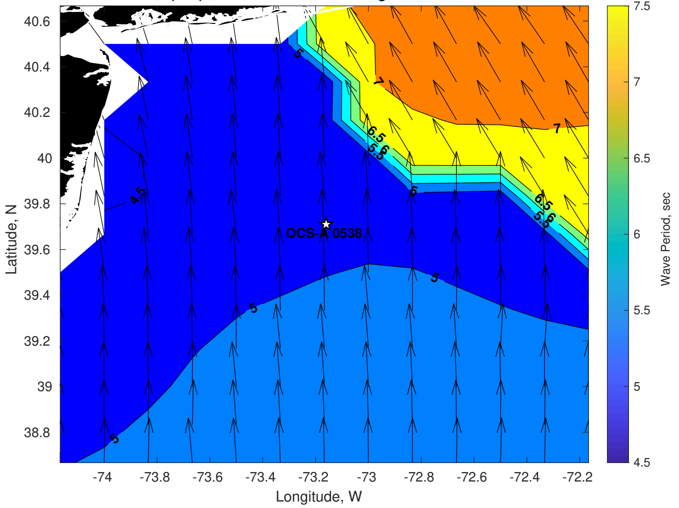
Wave Period (sec) for OCS-A 0538 at 03-Aug-2024 00:00:00
