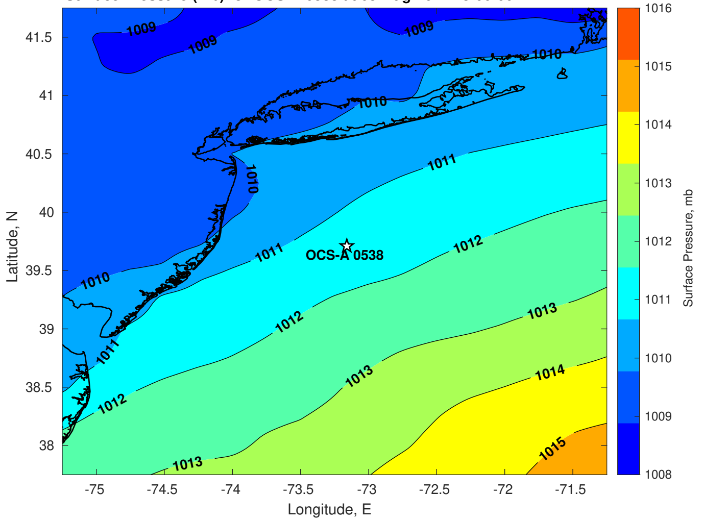
Surface Pressure (mb) for OCS-A 0538 at 03-Aug-2024 18:00:00
