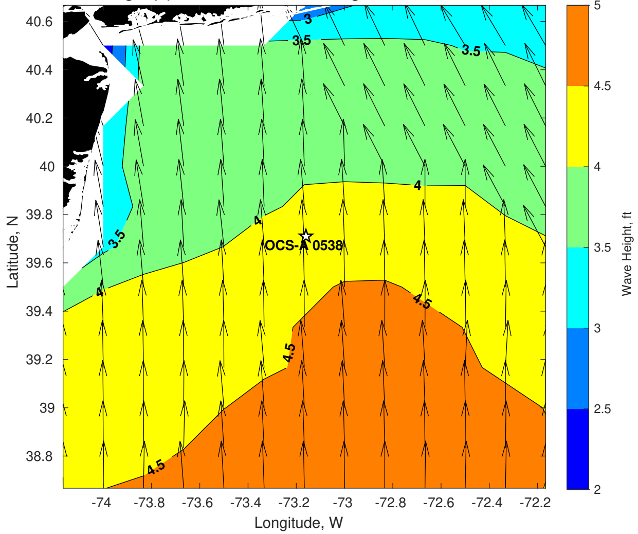
Wave Height (ft) for OCS-A 0538 at 03-Aug-2024 00:00:00
