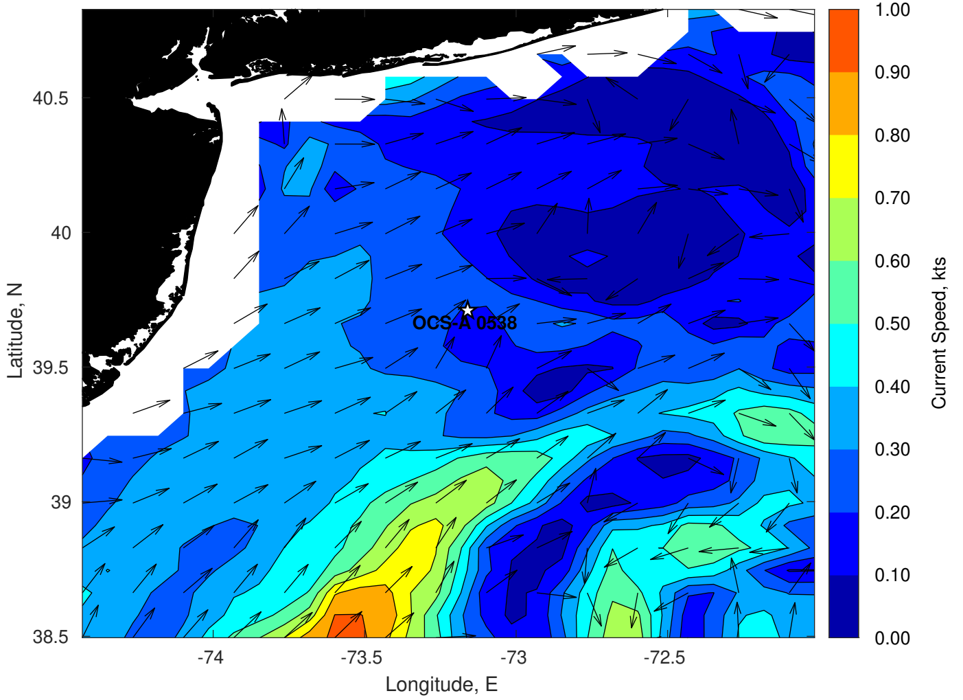
Surface Currents for OCS-A 0538 at 10-Jun-2023 00:00:00
