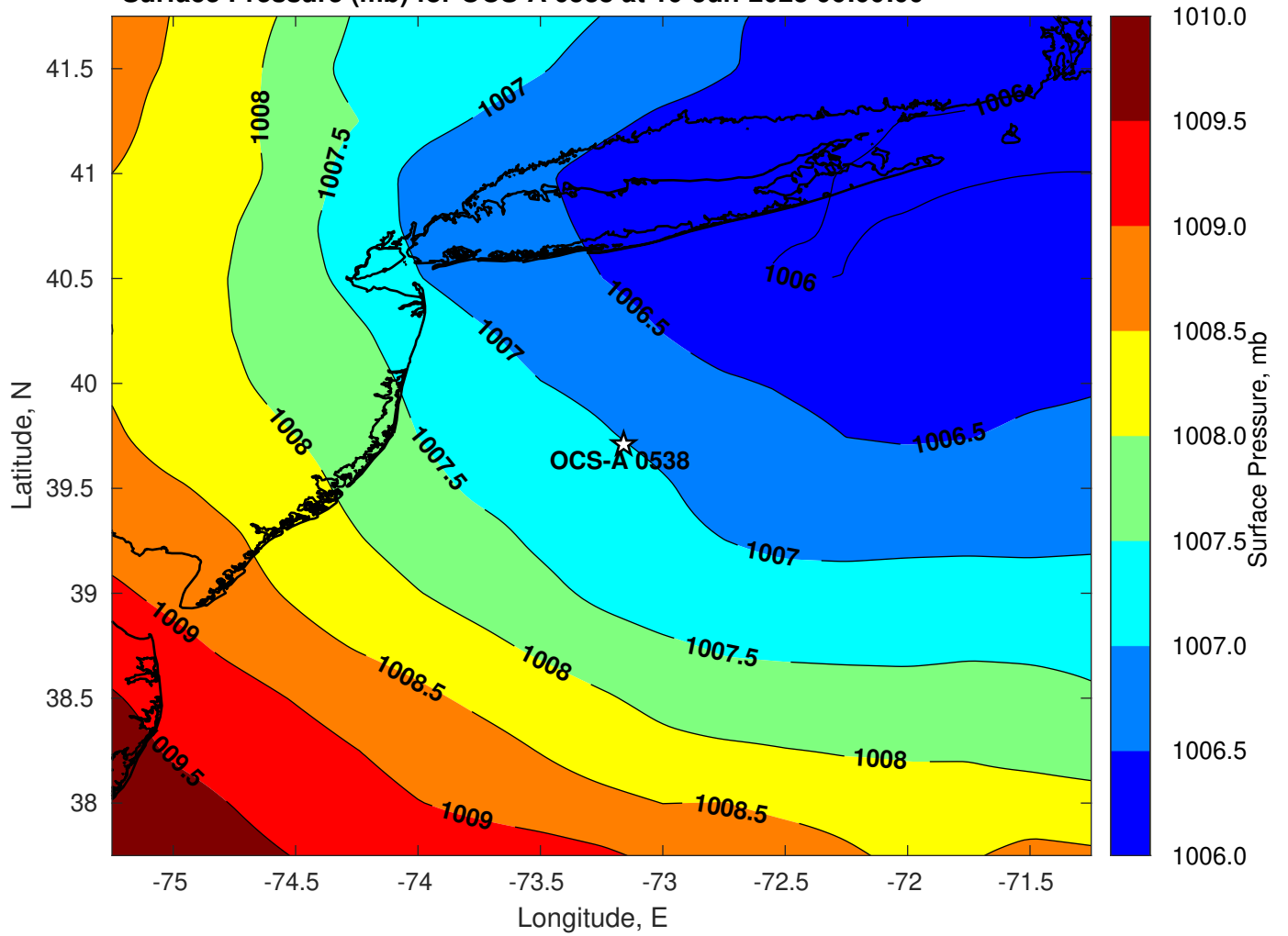
Surface Pressure (mb) for OCS-A 0538 at 10-Jun-2023 06:00:00
