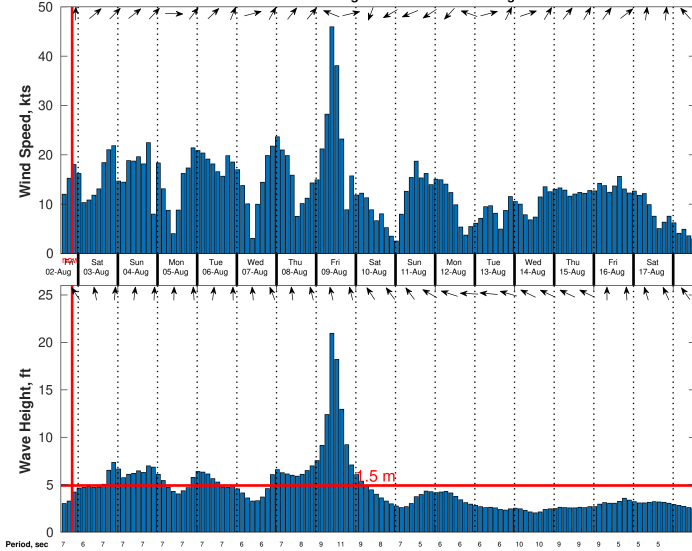
Wind & Wave Forecast for OCS-A 0538 from 02-Aug-2024 14:00:00 to 18-Aug-2024 14:00:00
