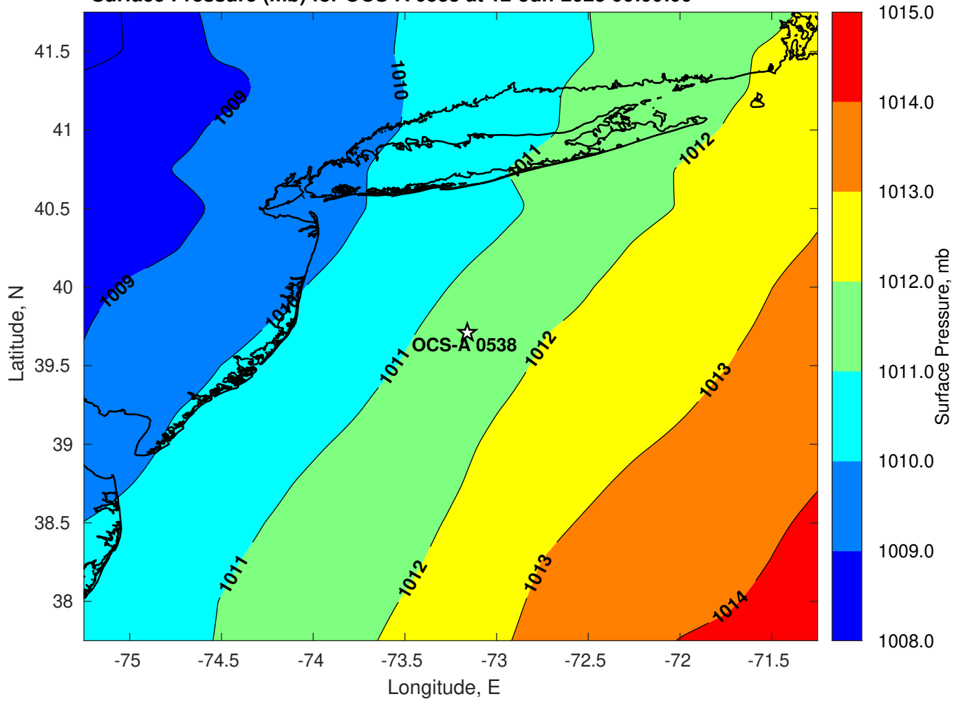
Surface Pressure (mb) for OCS-A 0538 at 12-Jun-2023 06:00:00
