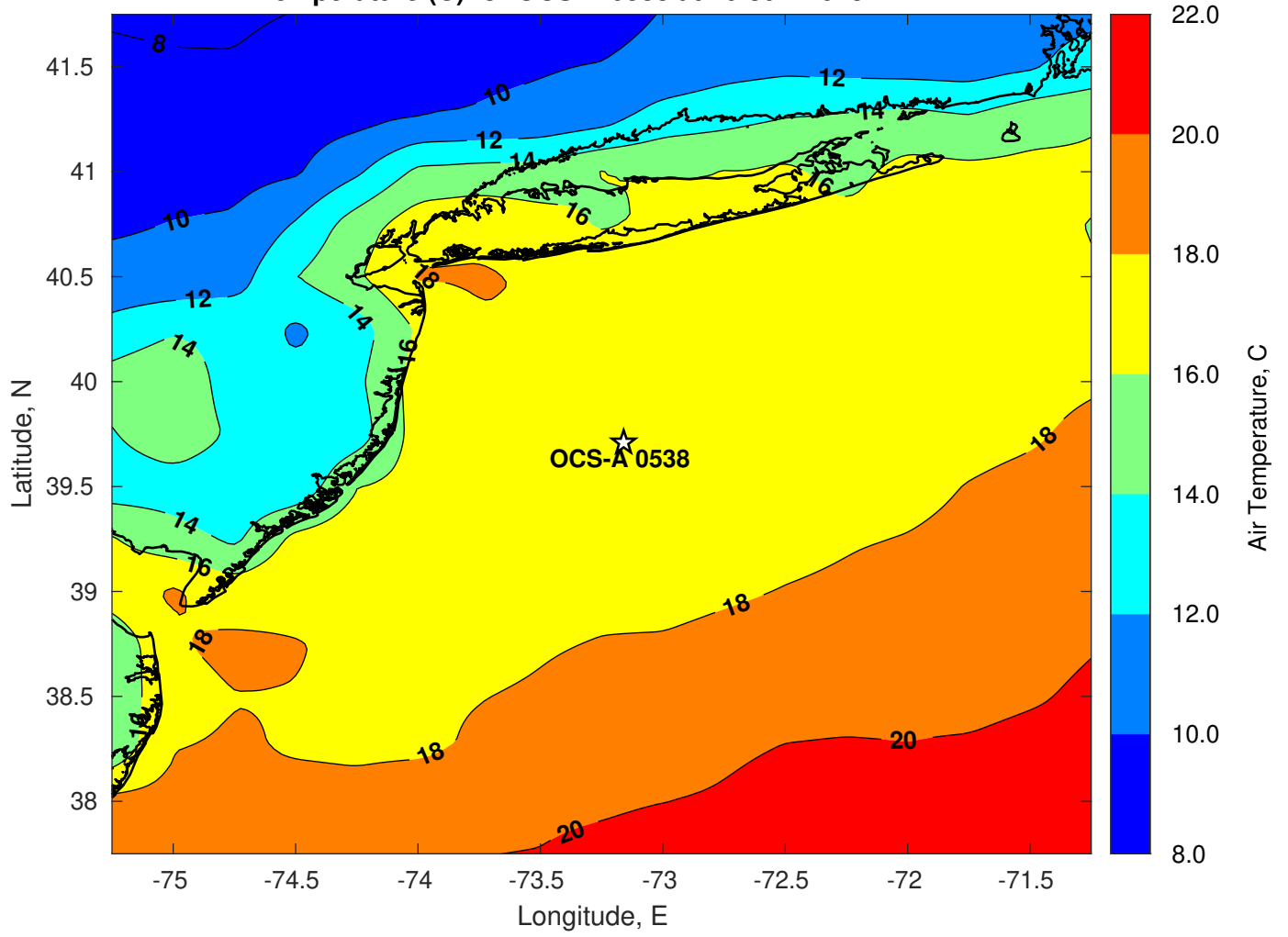
Air Temperature (C) for OCS-A 0538 at 10-Jun-2023
