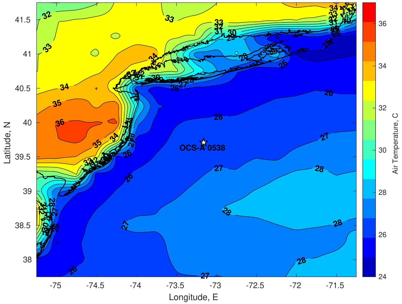
Air Temperature (C) for OCS-A 0538 at 02-Aug-2024
