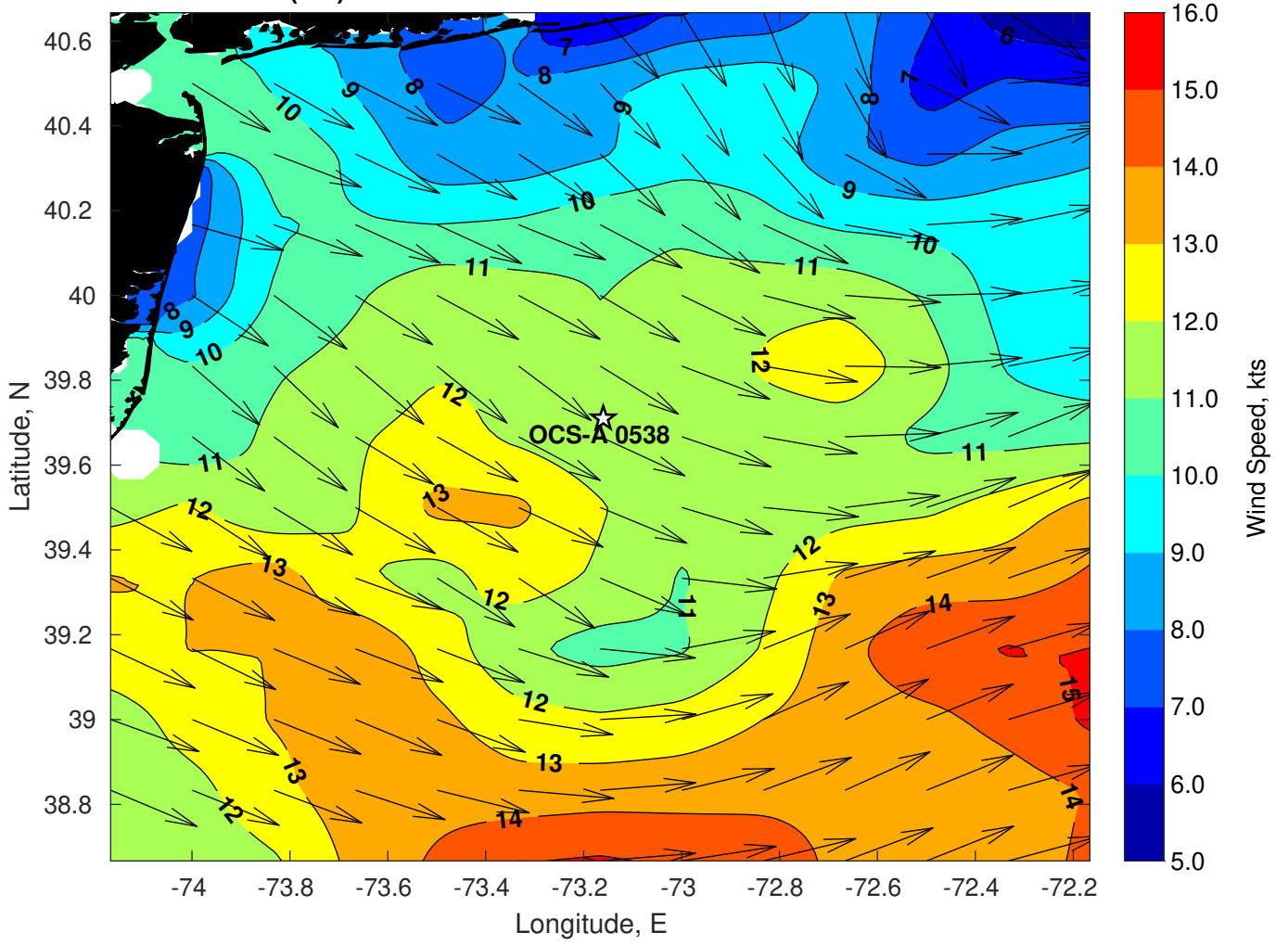
Winds (kts) for OCS-A 0538 at 10-Jun-2023 06:00:00
