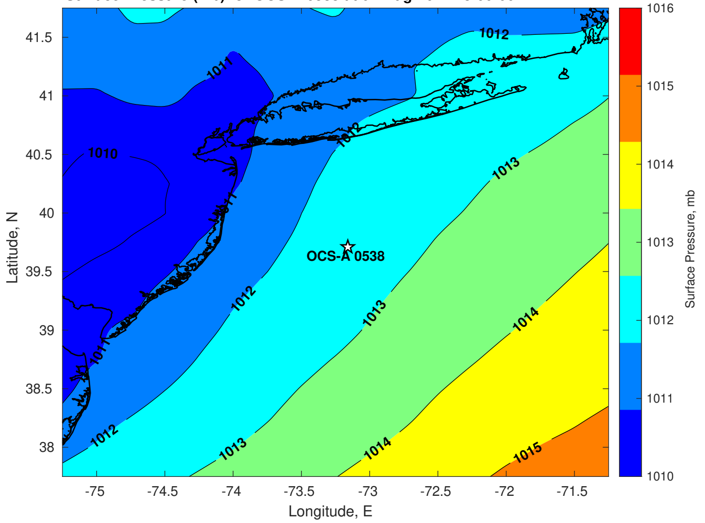
Surface Pressure (mb) for OCS-A 0538 at 02-Aug-2024 18:00:00
