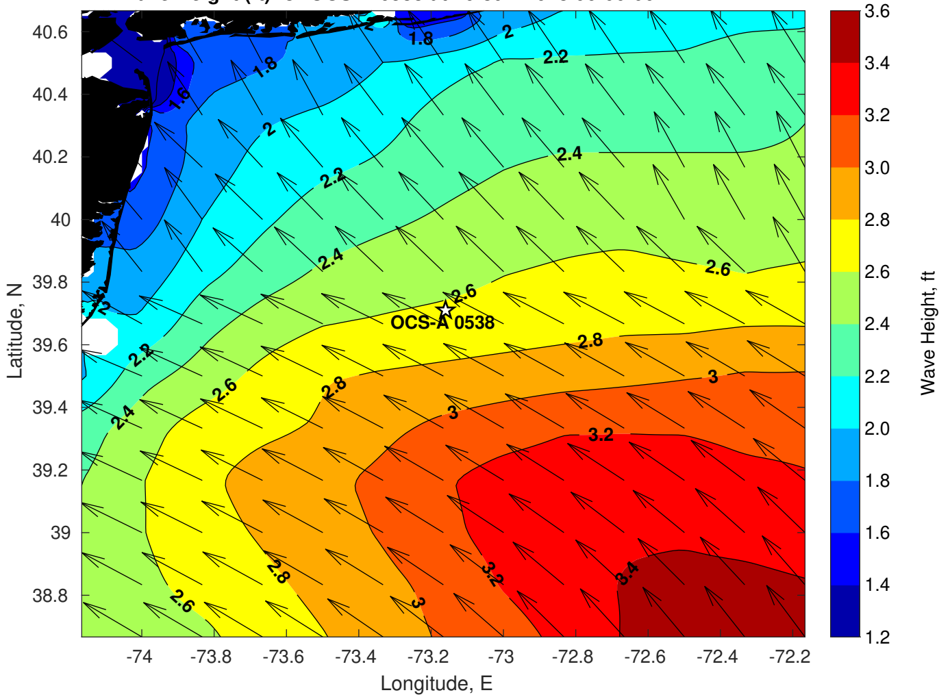
Wave Height (ft) for OCS-A 0538 at 10-Jun-2023 06:00:00
