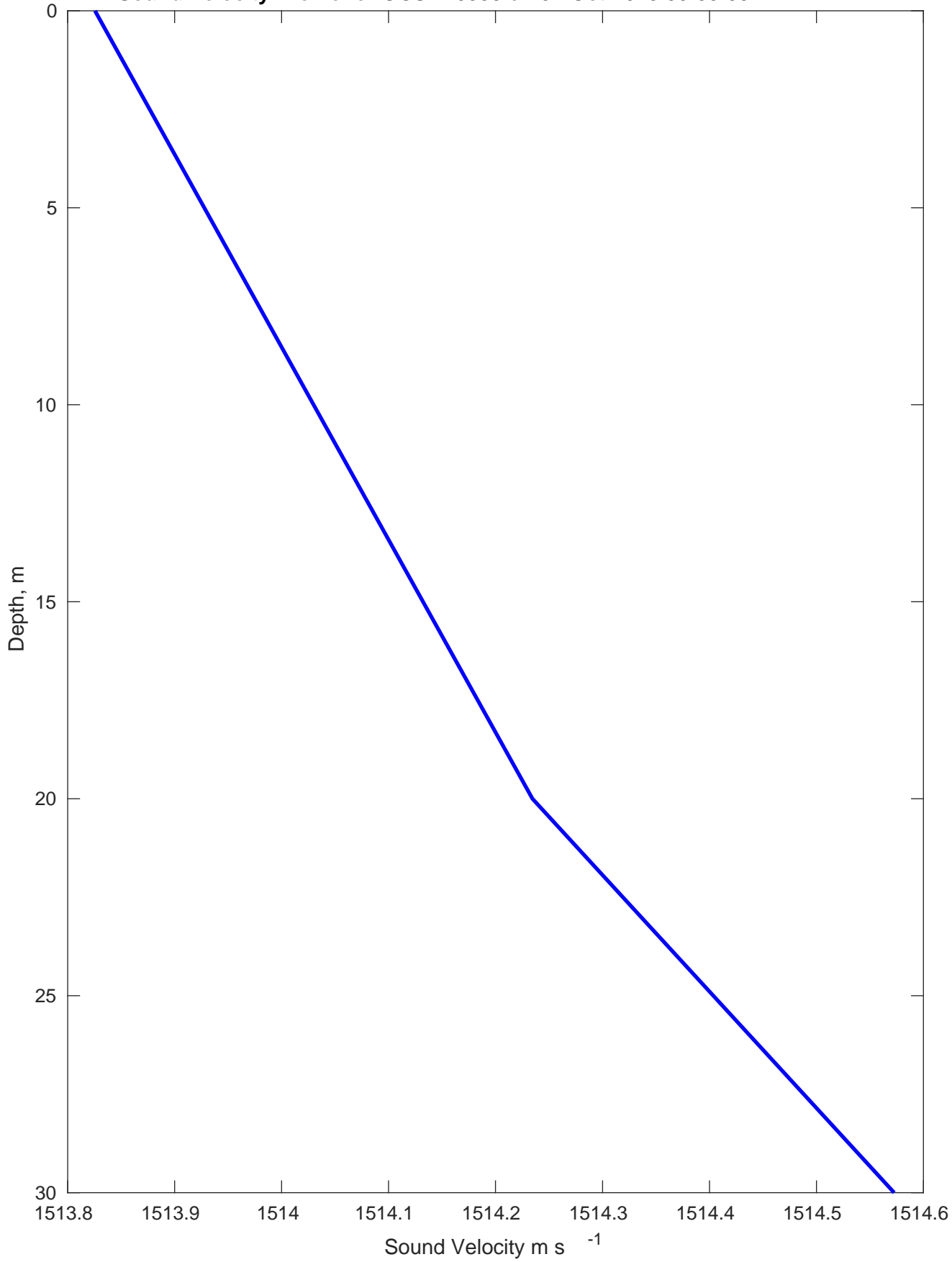
Sound Velocity Profile for OCS-A 0538 on 01-Oct-2023 00:00:00
