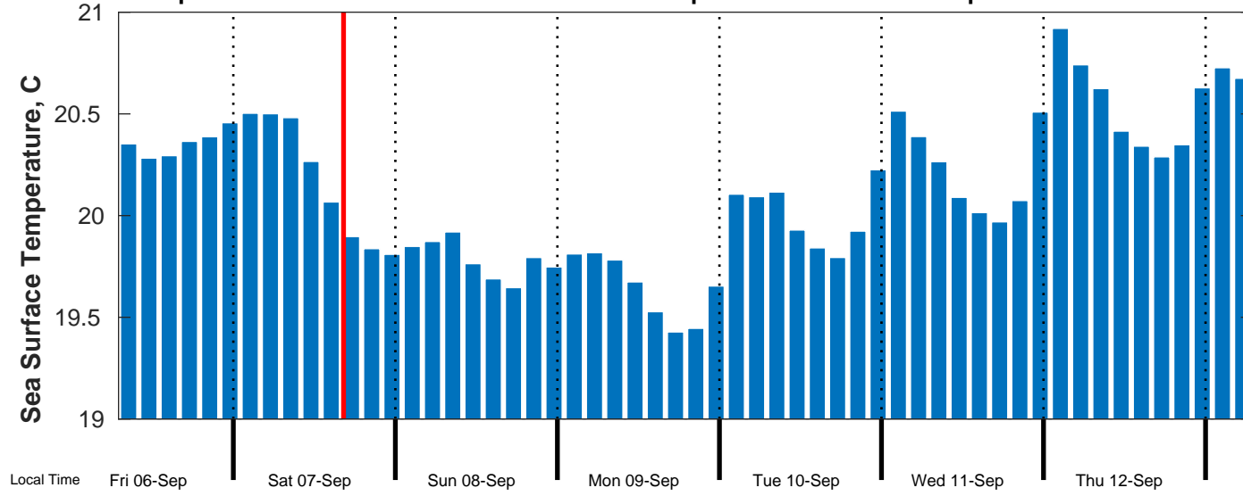
Sea Surface Temperature Forecast for OCS-A 0538 from 07-Sep-2024 00:00:00 to 14-Sep-2024 00:00:00
